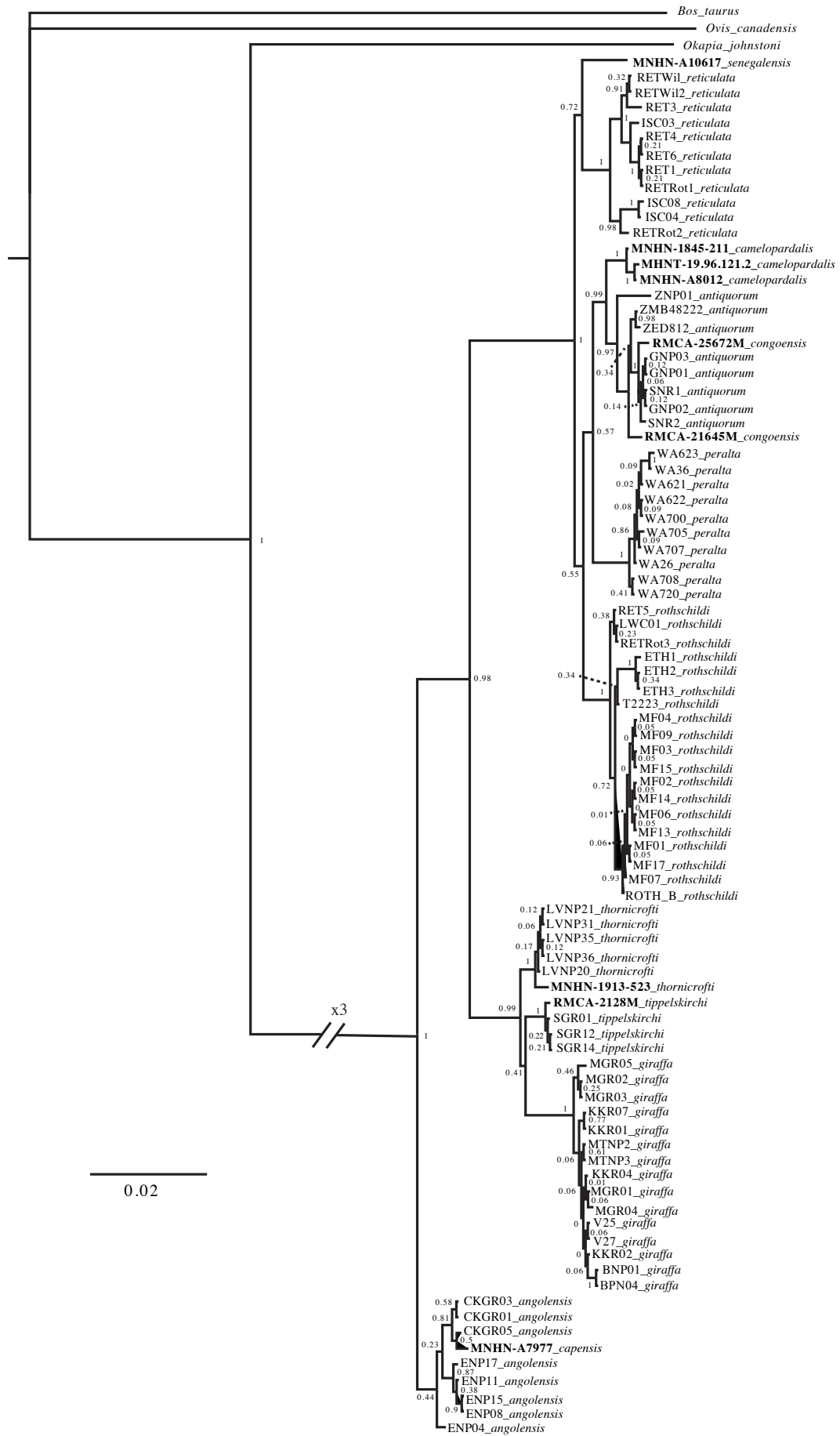
Supplementary file 4. Bayesian tree from the analysis of the mitochondrial fragment (1.776 bp, cytochrome b and the partial 5' region) including 88 giraffe individuals and three outgroup taxa. The posterior probability values are indicated for each node. Museum specimens are highlighted in bold.
