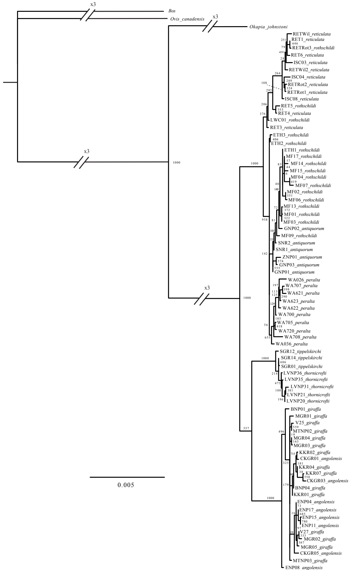
Supplementary file 7. PhyML tree from the Maximum Likelihood analysis of the concatenated alignment of 21 nuclear markers (17.275 bp) for 75 giraffes and three outgroup taxa. The bootstrap values are indicated for each node.
