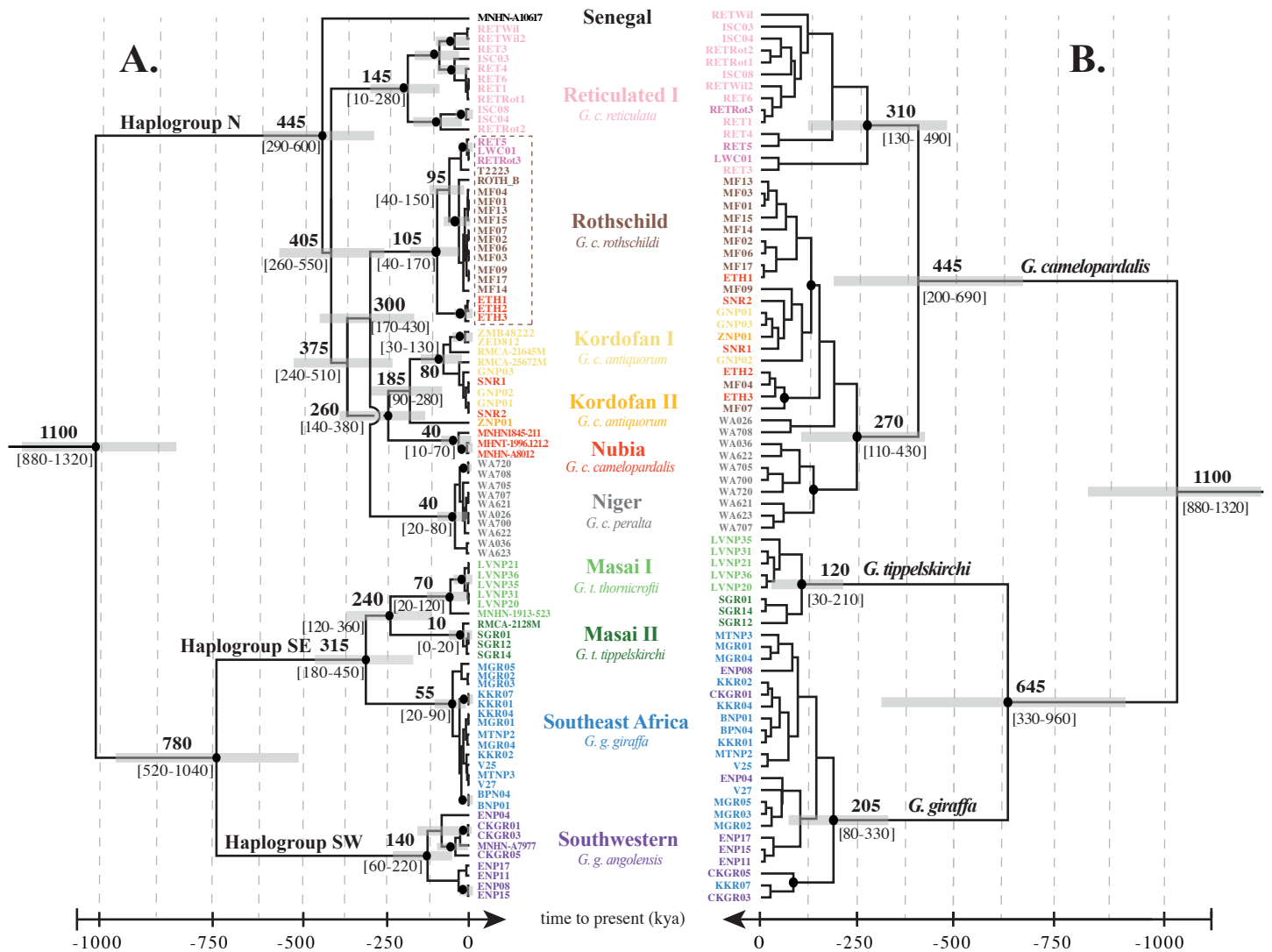
Supplementary file 8. Comparison of mitochondrial and nuclear divergence time estimates. A. Chronogram inferred from the mtDNA-91T dataset using BEAST v.1.8.4 (Drummond et al. 2012). Divergence time estimates are reported for the nodes supported by PP \geq 0.95 (black circles). B. Chronogram inferred from the nuDNA-78T dataset using BEAST v.1.8.4 (Drummond et al. 2012). Divergence time estimates are reported for the nodes found in concordance with the mtDNA chronogram and nodes discussed in the text. In both chronograms 95% confidence intervals are indicated by horizontal grey bars.
