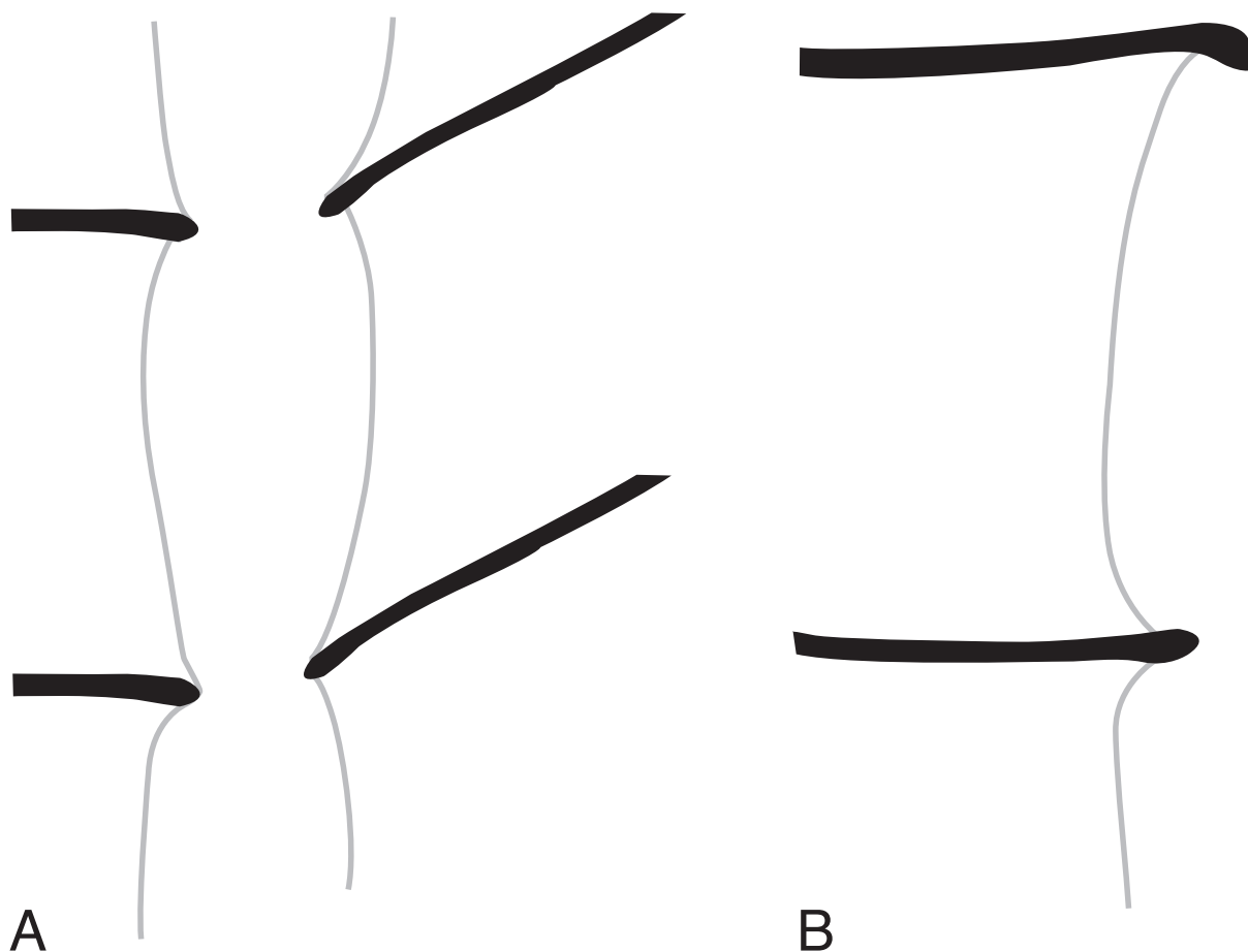
Fig. 21. Reconstruction of the details of the septal necks and connecting ring of Nathorstoceras sp. nov., Kallholn, Boda Limestone. A. Nathorstoceras kallholnense sp. nov., PMU 26729, holotype. B. Nathorstoceras adnatum sp. nov., PMU 26733, holotype.
