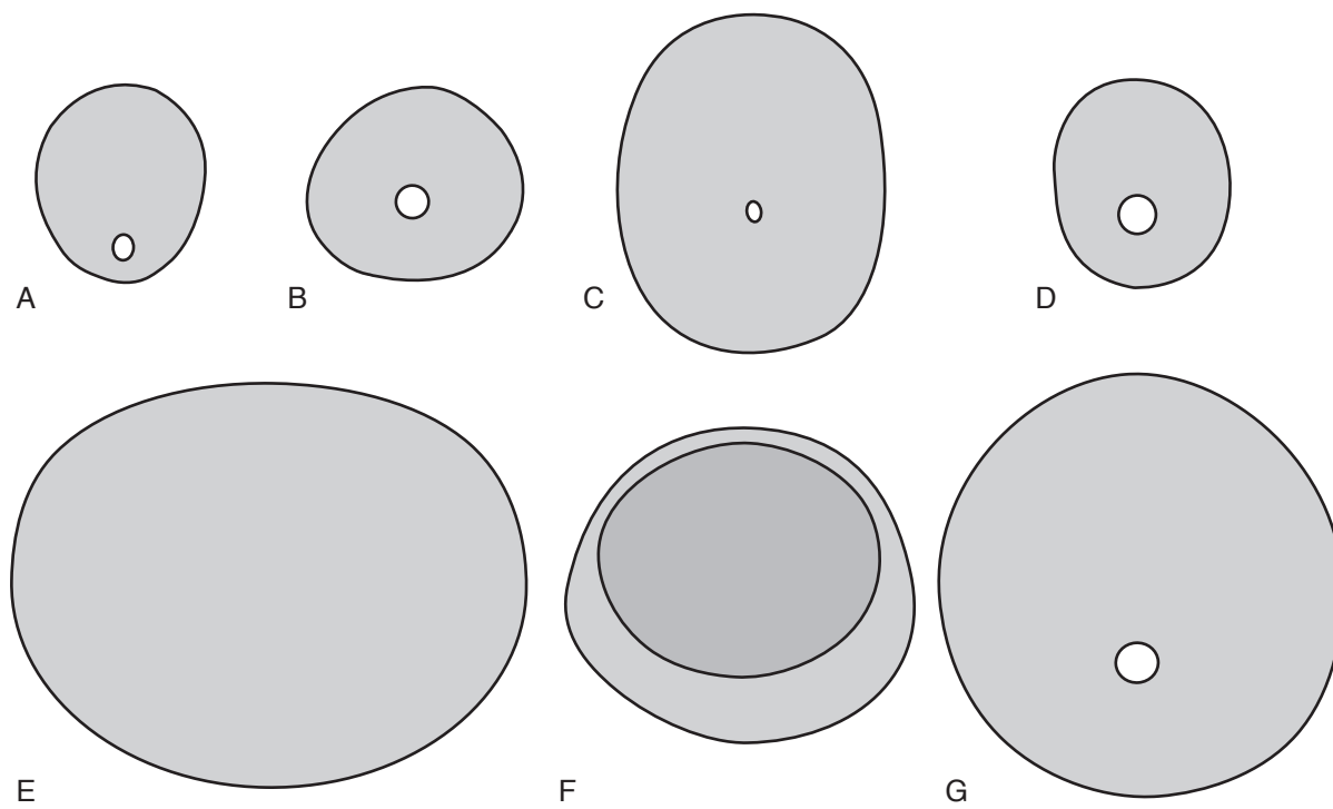
Fig. 10. Camera lucida drawings of cross sections of selected Boda Limestone cephalopods. A. Cyrtorizoceras thorslundi sp. nov., PMU 26657, Osmundsberget, mature body chamber. B. Tyrioceras cf. kjaerulfi Strand, 1934, PMU 26897, Kallholn. C. Nathorstoceras adnatum sp. nov., PMU 26733, holotype, Kallholn. D. Nathorstoceras kallholnense sp. nov., PMU 26729, holotype. E. Redpathoceras depressum sp. nov., PMU 26927, holotype, Kallholn, cross section of base of mature truncated conch. F. Schuchertoceras fryi sp. nov., PMU 24744, holotype, Kallholn, cross section of mature aperture (dark grey) and body chamber (medium grey). G. Redpathoceras bullatum sp. nov., PMU 26923, holotype, Kallholn, cross section of base of mature truncated conch. Prosiphuncular side directed downward in all figures. Siphuncles shown as white circles. Scale bar = 10 mm for all figures.
