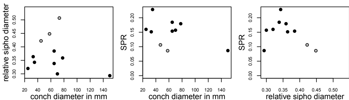
Fig. 3. Variation in relative siphuncle size, position and angle of expansion in Cameroceras hasta (Eichwald, 1860) (grey points) and Cameroceras turrisoides sp. nov. SPR = the minimum distance of the connecting ring from the conch margin, divided by the corresponding conch height.
