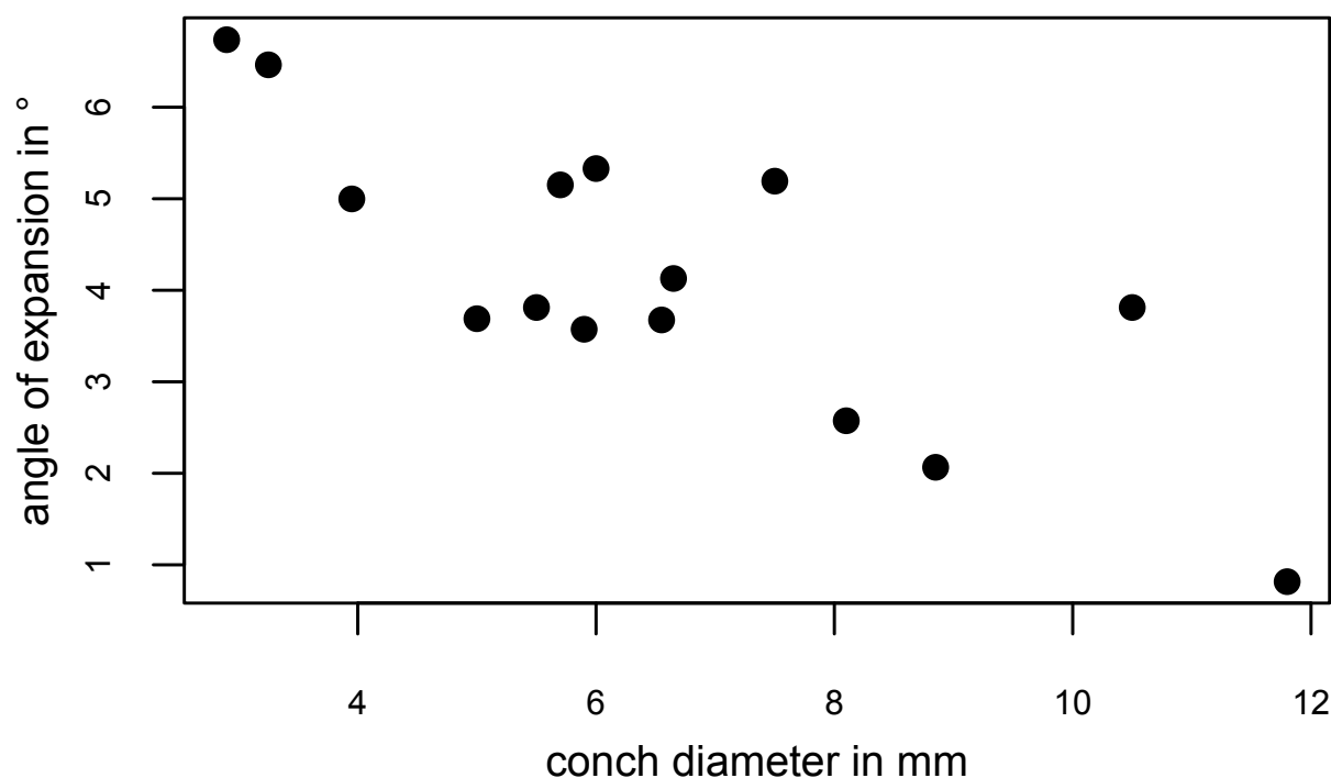
Fig. 27. Angle of expansion of 15 measured specimen of Isorthoceras cf. elongatocinctum (Portlock, 1843), Boda Limestone, Late Katian, Dalarna, Sweden.
