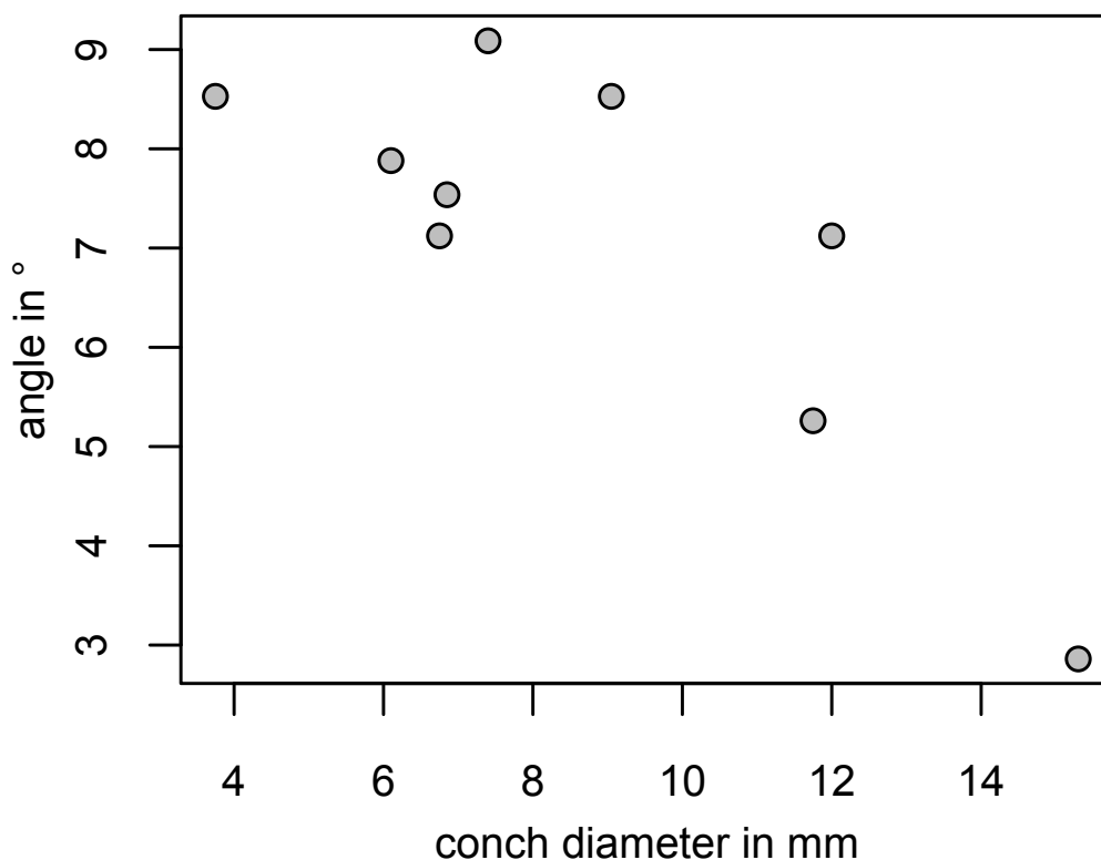
Fig. 25. Variability of the angle of expansion in fragments of different diameters of Isorthoceras angelini sp. nov. Note the tendency of decreasing angle of expansion with diameter. The adult diameter is reached at ca. 15 mm.
