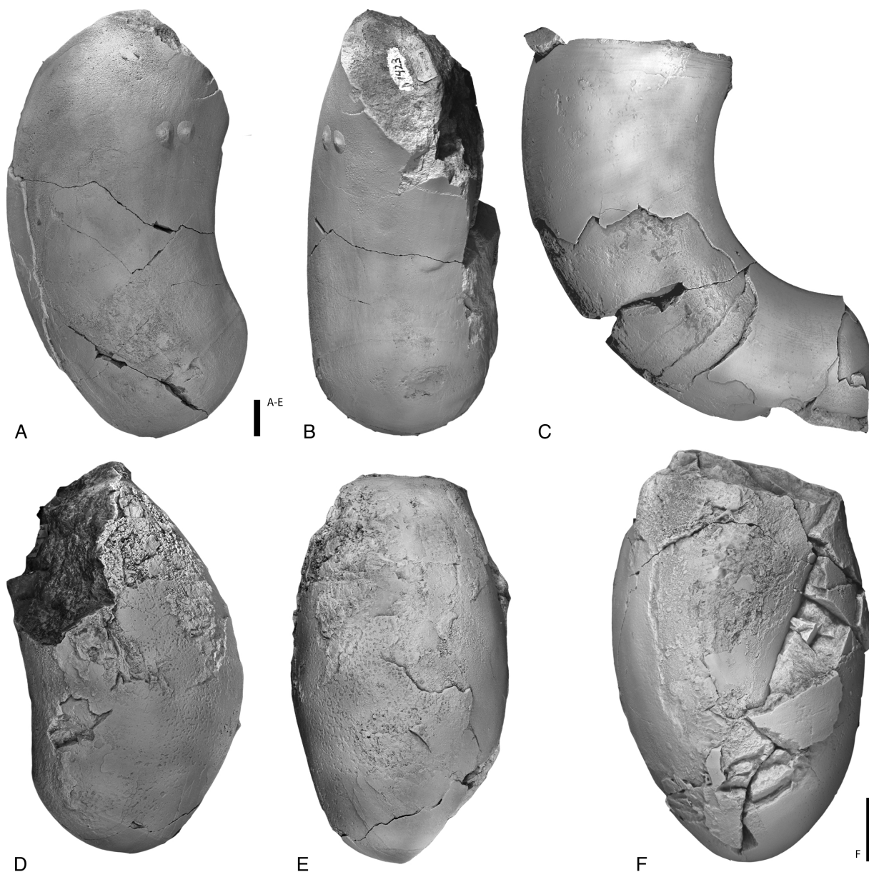
Fig. 39. Ascocerida and Uranoceratidae of the Boda Limestone. A-B. Redpathoceras bullatum sp. nov. A. PMU 26923, holotype, Kallholn; mature truncated body chamber, lateral view. B. Same specimen, view from antisiphuncular side. C. Warburgoceras longitudinale (Angelin in Angelin & Lindström, 1880) comb. nov., NRM-PZ Mo 154065, Unskarsheden; mature body chamber and part of phragmocone in lateral view. D-E. Probillingsites scandinavicum sp. nov., PMU 26922, holotype, Kallholn. D. Mature truncated body chamber, lateral view. E. Same specimen, view from prosiphuncular side. F. Schuchertoceras fryi sp. nov., PMU 24744, holotype, Kallholn, lateral view. Scale bars: A-E = 10 mm; F = 10 mm.
