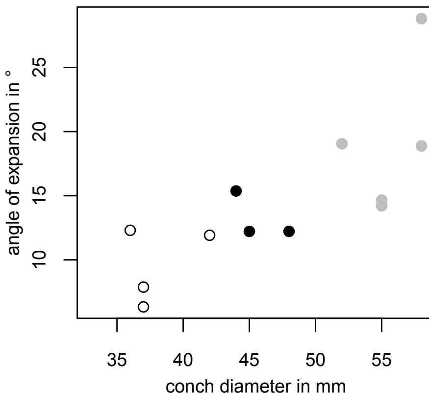
Fig. 42. Variation in angle of expansion in Redpathoceras Flower, 1963, Boda Limestone. R. magnum sp. nov. (grey dots); R. bullatum sp. nov. (black dots); R. depressum sp. nov. (black circles).
