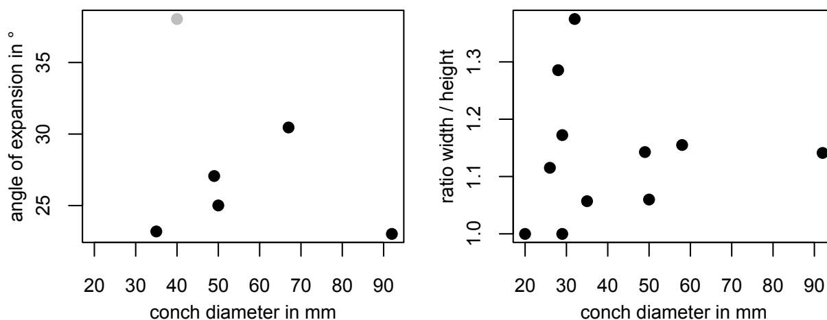
Fig. 38. Morphological variation of Siljanoceras gen. nov. Black dots = Siljanoceras varians sp. nov.; grey dot = Siljanoceras sp. A.
