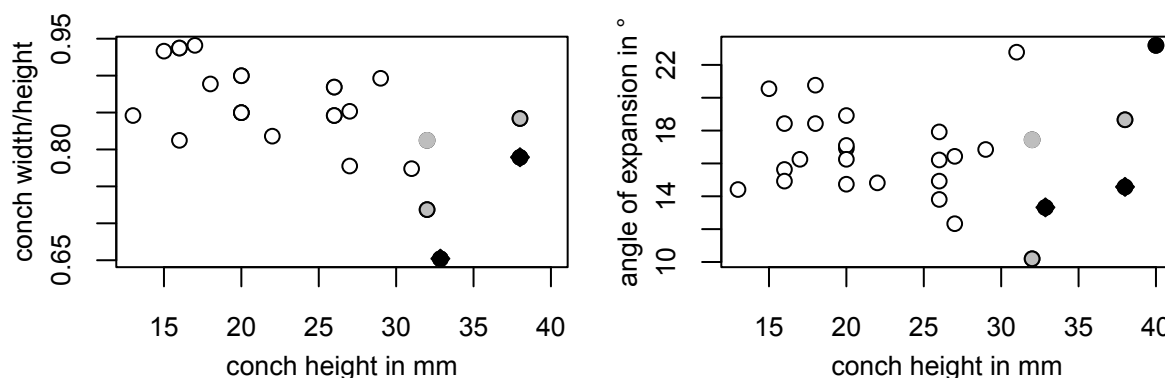
Fig. 11. Morphological variation of Beloitoceras sinuososeptatum (Roemer, 1861). Circles: specimens of the Boda Limestone. Black dot: type specimen of Beloitoceras siljanense Frye, 1987. Black diamonds: types of Beloitoceras heterocurvatum Strand, 1934. Grey dot: type specimen of Beloitoceras landerense Foerste, 1935. A distinction between B. siljanense and B. sinuososeptatum is impossible based on the available material.
