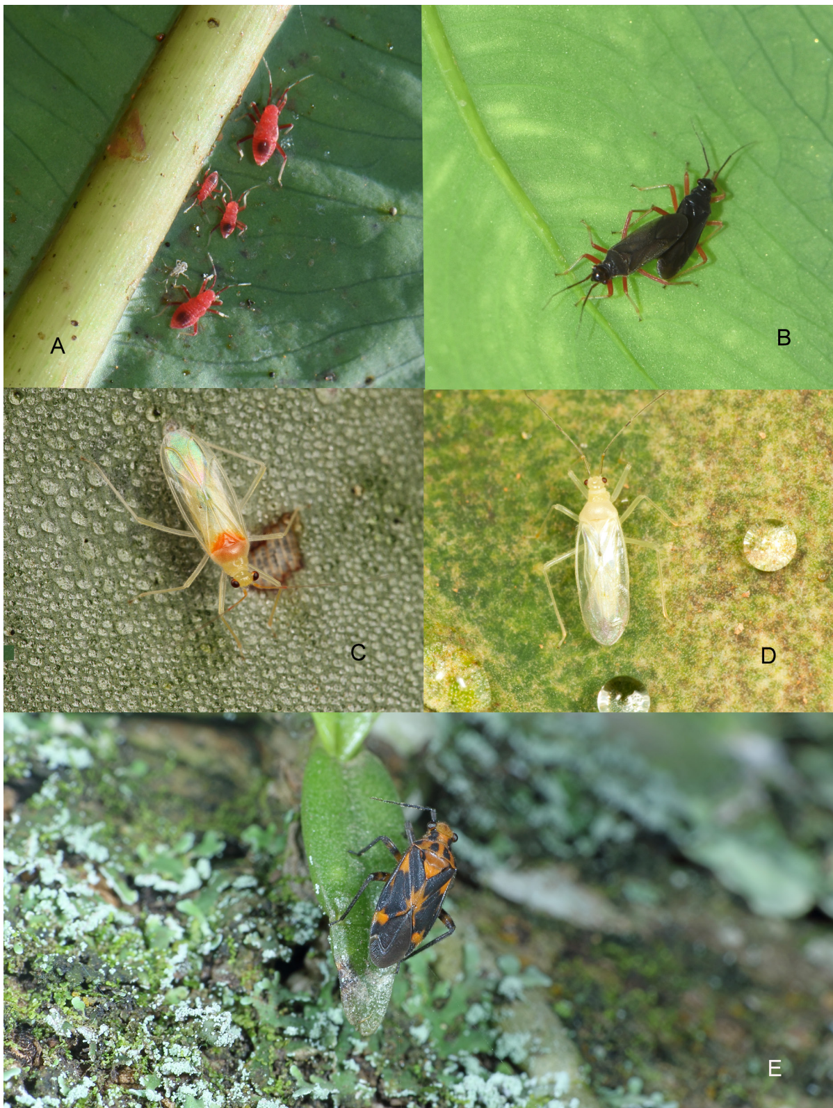
Fig. 27. Habitats and living specimens. A–B. Harpedona sanguinipes Distant, 1909 on Colocasia esculenta . A. Nymphs. B. Mating adults. C. Prodromus clypeatus Distant, 1904 on banana. D. Stonedahlia mishmiensis gen. et sp. nov. on Colocasia sp. E. Lopidolon dandeliensis sp. nov. on Diplocentrum recurvum . All specimens at UASB.
