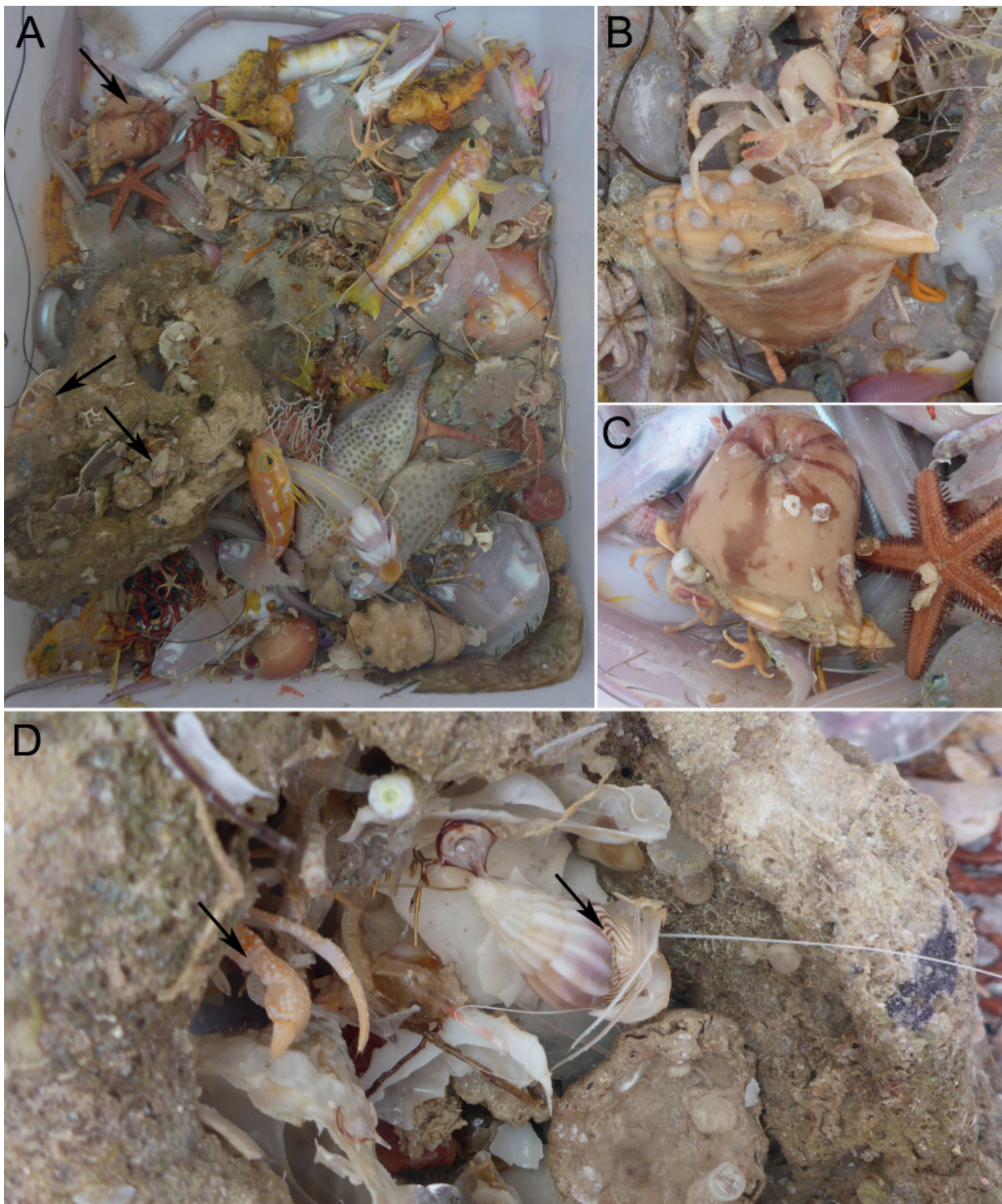
Fig. 5. Bottom trawl haul contents of KANADEEP Sta. CP4958 (Argo Bank), collection locality of one of the paratypes of Aretopsis sandybrucei sp. nov. A. General view of haul contents, with black arrows pointing to several hermit crabs (Paguridae). B–C. Hermit crab, possibly Diacanthurus sp. (Paguridae), carrying a large gastropod shell also harbouring a sea anemone. D. Two hermit crabs of the family Paguridae. Photographs by Dr Sarah Samadi.
