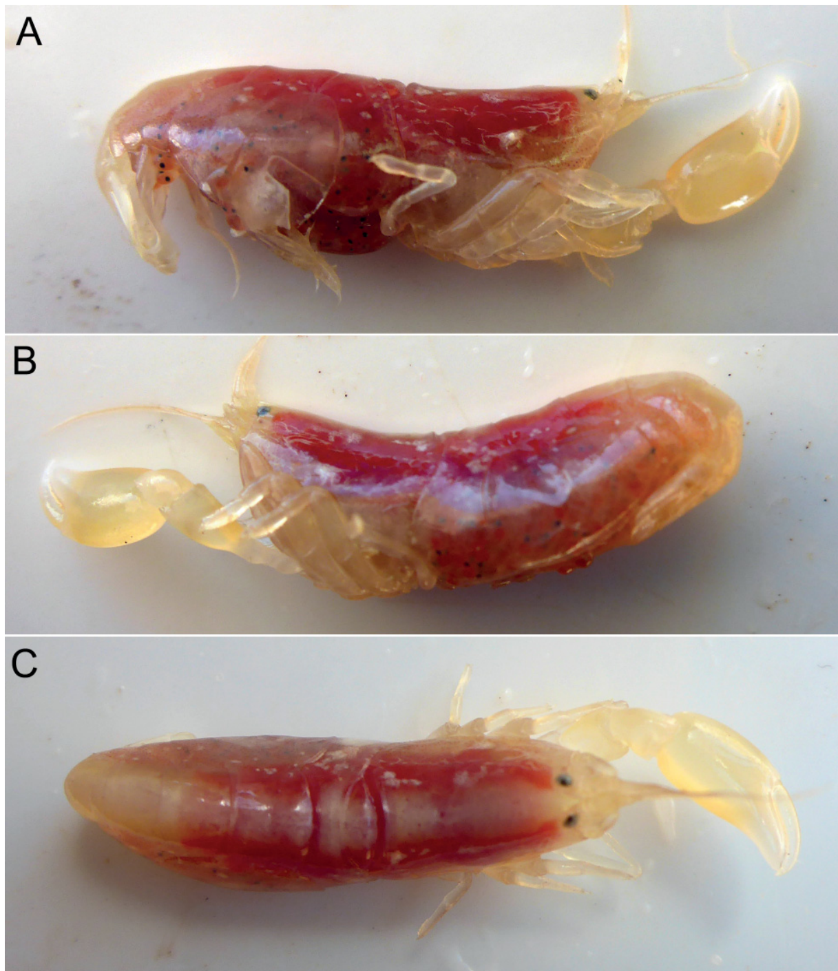
Fig. 4. Aretopsis sandybrucei sp. nov., paratype, ovigerous ♀ (cl 6.58 mm) from Argo Bank, Coral Sea (MNHN-IU-2017-2770), shrimp missing right (minor) cheliped, photographed shortly after collection. A. Right lateral view. B. Left lateral view. C. Dorsal view. Photographs by Dr. Sarah Samadi.
