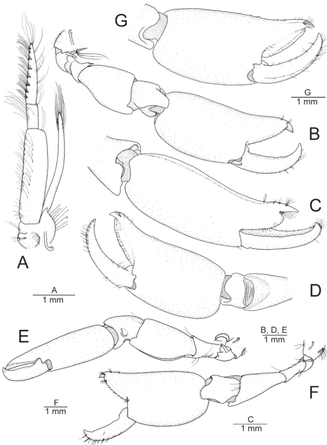
Fig. 2. Aretopsis sandybrucei sp. nov., holotype, ♂ (cl 5.31 mm) from Capel Bank, Coral Sea (MNHN-IU-2017-2924). A. Third maxilliped, lateral view. B. Right (major) cheliped, lateral view. C. Same, distal portion of carpus and chela, dorsolateral view. D. Same, distal portion of merus, carpus and chela, mesial view. E. Left (minor) cheliped, dorsolateral view. F. Same, chela fingers open, lateral view. G. Same, chela, mesial view.
