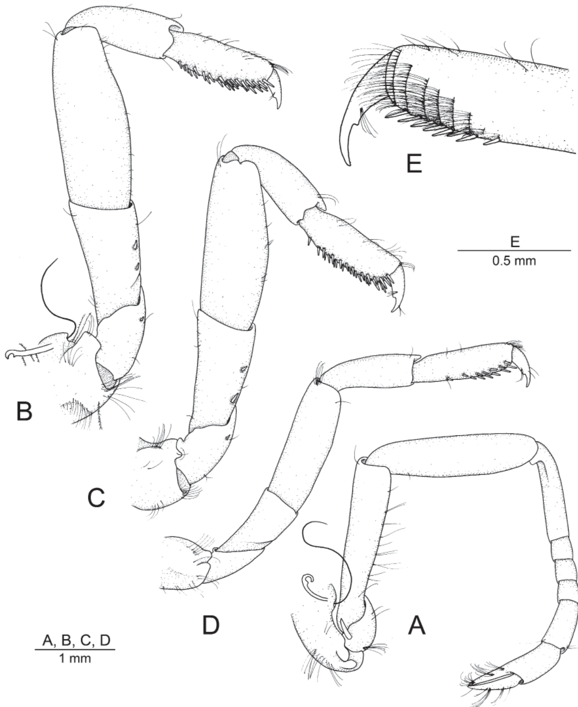
Fig. 3. Aretopsis sandybrucei sp. nov., holotype, ♂ (cl 5.31 mm) from Capel Bank, Coral Sea (MNHN-IU-2017-2924). A. Second pereiopod, lateral view. B. Third pereiopod, lateral view. C. Fourth pereiopod, lateral view. D. Fifth pereiopod, lateral view. E. Same, distal portion of propodus and dactylus, mesial view.
