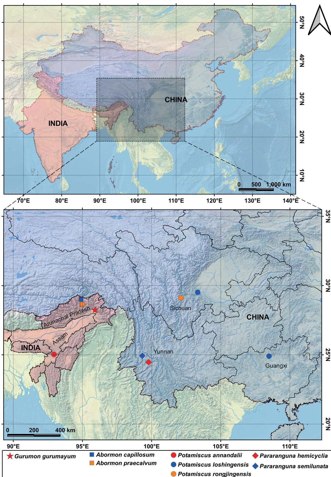
Fig. 5. Map showing India, China and distribution of the species of Gurumon gen. nov., Abormon Mitra, Pati & Ng, 2021, Pararanguna Dai & Chen, 1985, and Potamiscus Alcock, 1909.
