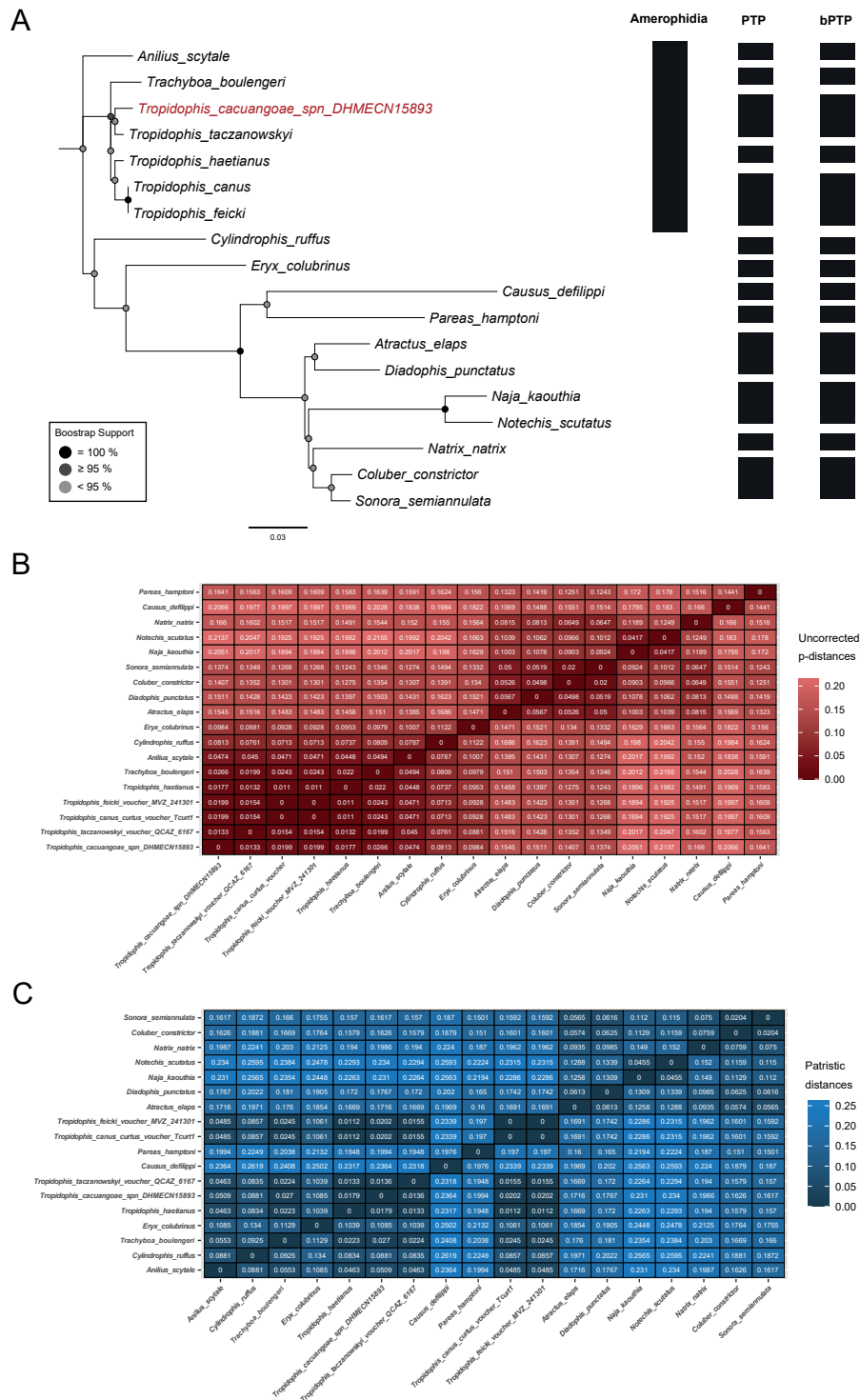
Fig. 2. Phylogenetic relationships of amerophid snakes, based on nuclear data. A. Maximum likelihood topology ( \ln L = -2175.559394 ), based on neurotrophin-3 gene fragments, scale bar of substitution rates, bars indicate Amerophidia clade, Poisson Tree Process (PTP) and Bayesian Poisson Tree Process (bPTP) coalescent-based species delimitation analyses. B. Uncorrected p-distances. C. Patristic distances as inferred for maximum likelihood tree.
