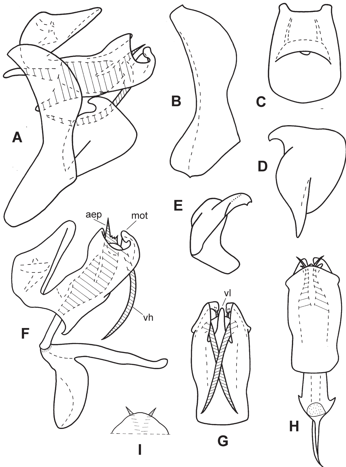
Fig. 6. Oceatra litoralis gen. et sp. nov., holotype, ♂ (MMBC), terminalia. A. Genital block, lateral view. B. Pygofer, lateral view. C. Anal tube, dorsal view. D. Style, lateral view. E. Style, dorsal view. F. Penis, connective, and anal tube, lateral view. G. Penis, ventral view. H. Penis and connective, dorsal view. I. Apex of penis, dorsal view. Abbreviations: aep = apical aedeagal process; mot = mushroom-shaped outgrowth of phallobase; vh = ventral aedeagal hooks; vl = ventral phallobase lobe. Not to scale.
