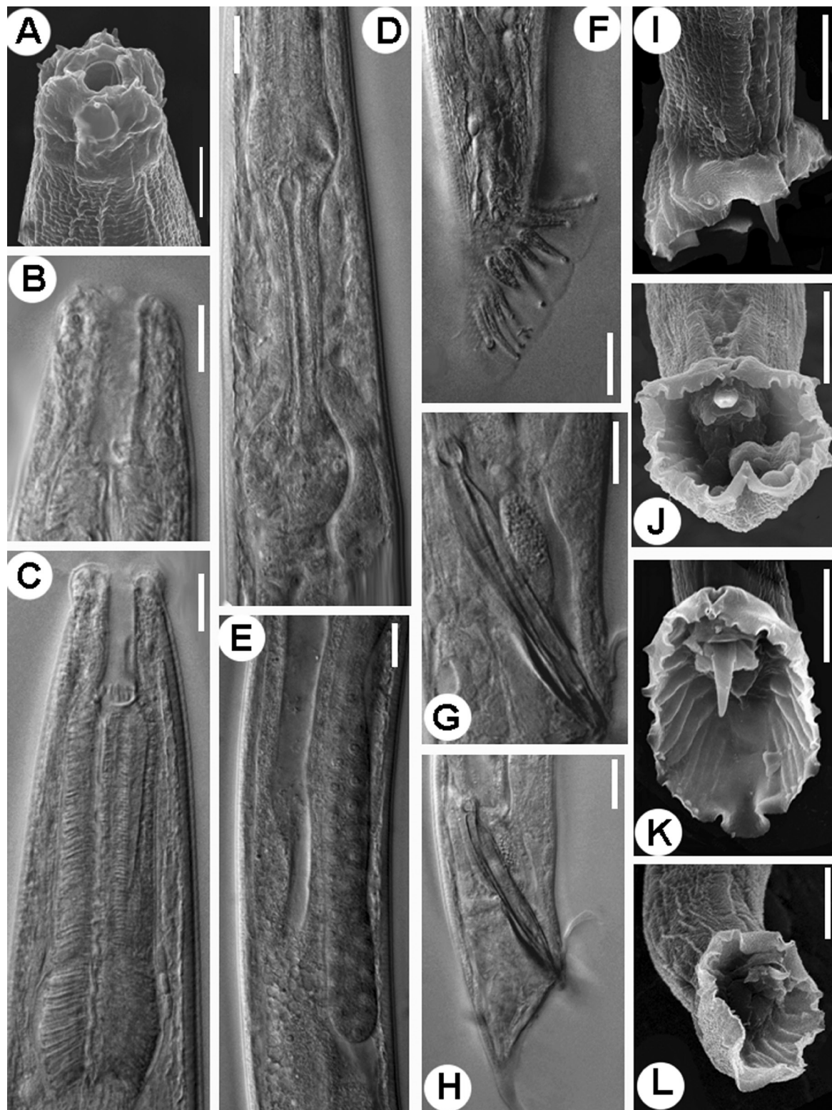
Fig. 3. Pelodera indica sp. nov., paratype, ♂ (AMU/ZD/NC slide no. Pelodera indica sp. nov./NIT/ctrs/2–15). A. Anterior region (scanning electron microscopy). B. Anterior end. C. Anterior pharyngeal region. D. Posterior pharyngeal region. E. Ovarian flexure of anterior genital branch. F–H. Posterior region showing spicules and gubernaculum. I–L. Tail region showing bursa and genital papillae (scanning electron microscopy). Scale bars = 10 \mu m.
