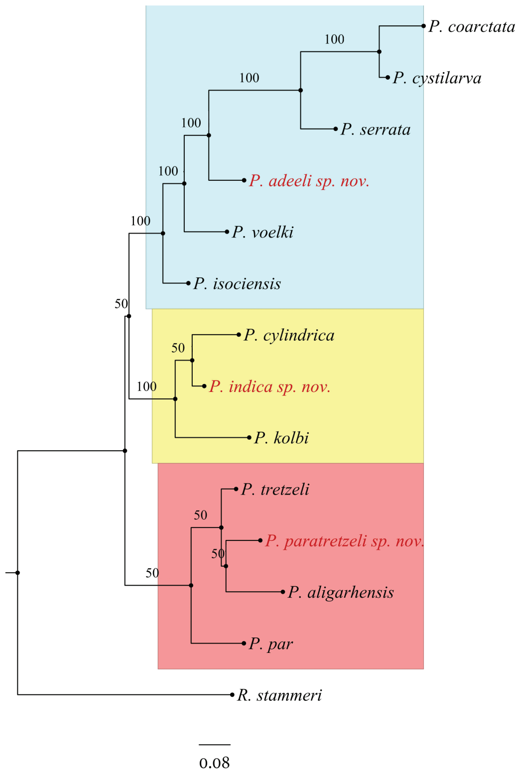
Fig. 15. Cladistic analysis of the species of genus Pelodera Schneider, 1866 ( coarctata group) indicating the position of the new species P. indica sp. nov., P. adeeli sp. nov. and P. paratretzeli sp. nov. within the genus. The evolutionary history was inferred in MrBayes ver. 3.1.2 (Huelsenbeck & Ronquist 2001) by using the Jukes Cantor (JC) model. The phylogenetic tree is supported by posterior probability values with minimum 50% majority rules.
