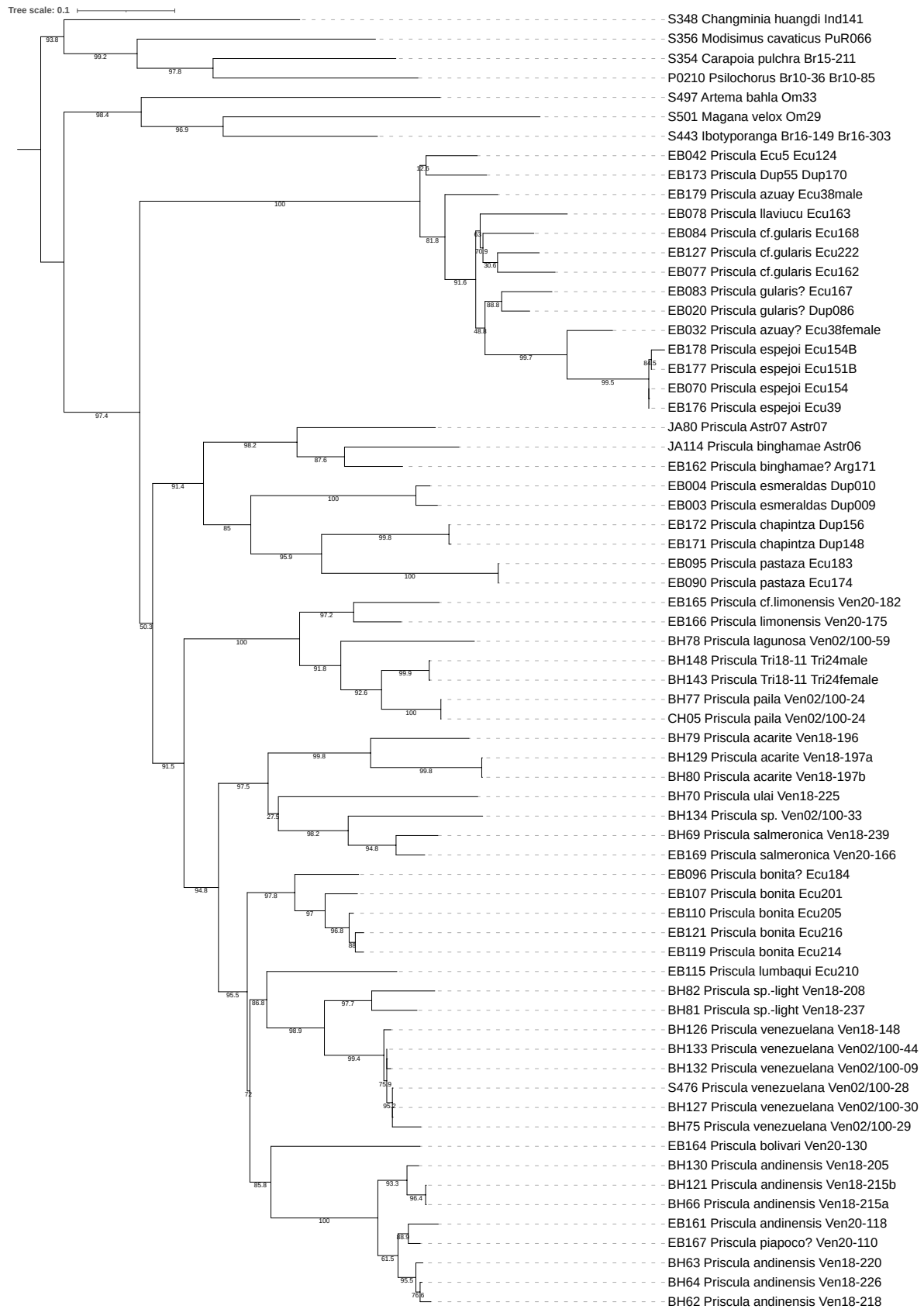
Figure S1. Maximum likelihood tree from ClipKIT_kpic-smart-gap-trimmed alignments and unpartitioned analysis using IQ-TREE. Numbers on the branches are SH-aLRT support (%). Best-fit model according to BIC for the reference tree: SYM+I+G4. https://doi.org/10.5852/ejt.2023.909.2351.10263
