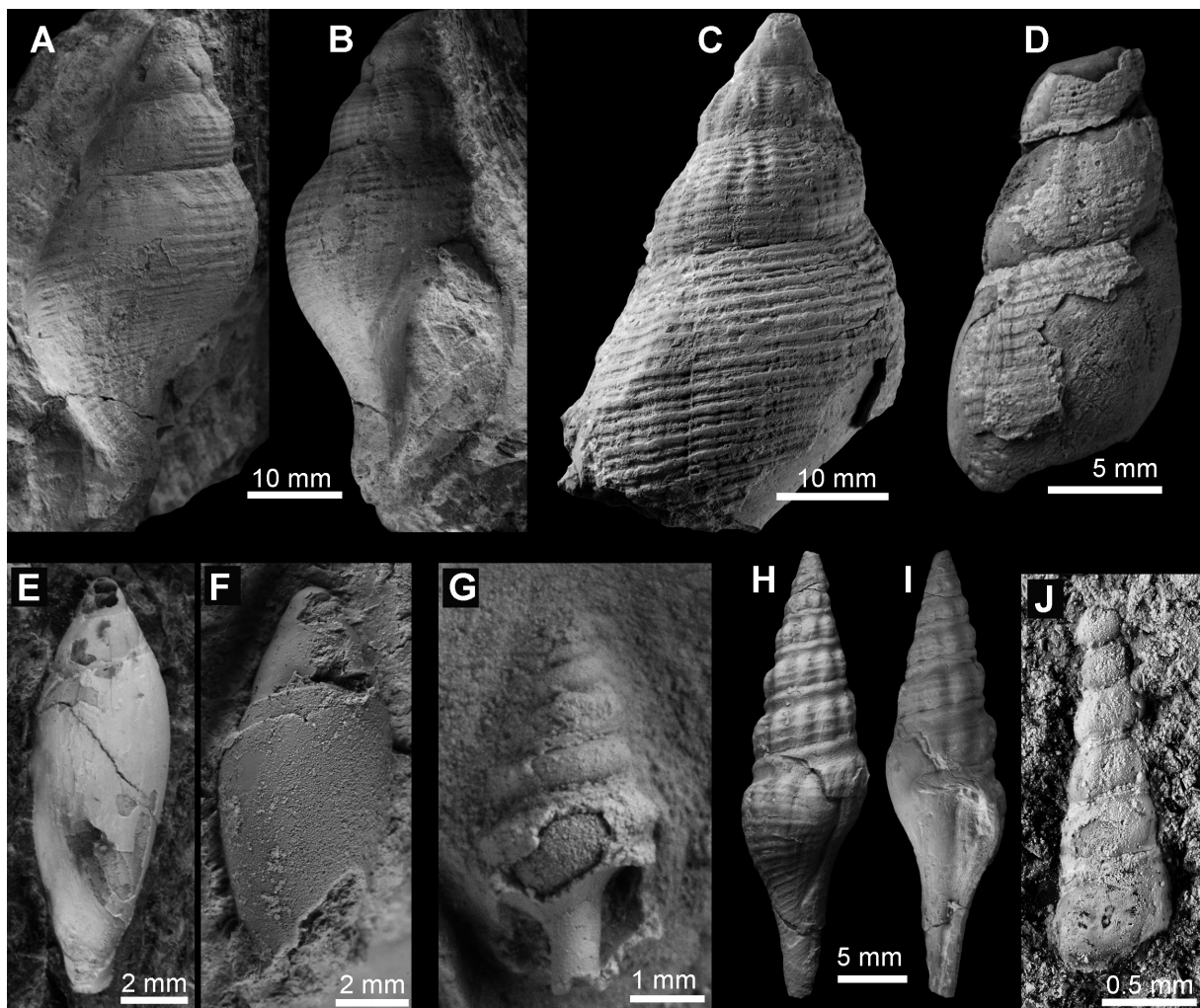
Fig. 7. Neogastropoda Wenz, 1938 and Heterobranchia Burmeister, 1837 from Miocene Calcarei a Lucina seep deposits in northern Italy. A–C. The eosiphonid Eosiphonid hoernesii (Bellardi, 1872). A–B. Specimen with well-preserved aperture, from Ca' Piantè (MSF 1070). C. Specimen showing details of spiral ornament, from Ca' Rovereti (NRM Mo 204839). D. The buccinid Neptunea? sp. from Le Colline (MSF 2359). E–F. The olivid Olivella longispira Bellardi, 1882. E. From Le Colline (MSF 1202). F. From Guzzano (MGGC 22310). G. The turrid Turris citima (Bellardi, 1877), from Ca' Cavalmagra (MSF 1307). H–I. The turrid Turricula sp., from Ca' Piantè (MSF 1081). J. The pyramidellid (Heterobranchia) Turbonilla sp., from Ca' Cavalmagra (MSF 1305).
