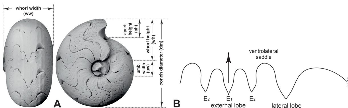
Fig. 3. The morphological terms used in the descriptions of the ammonoid conchs and suture lines.
