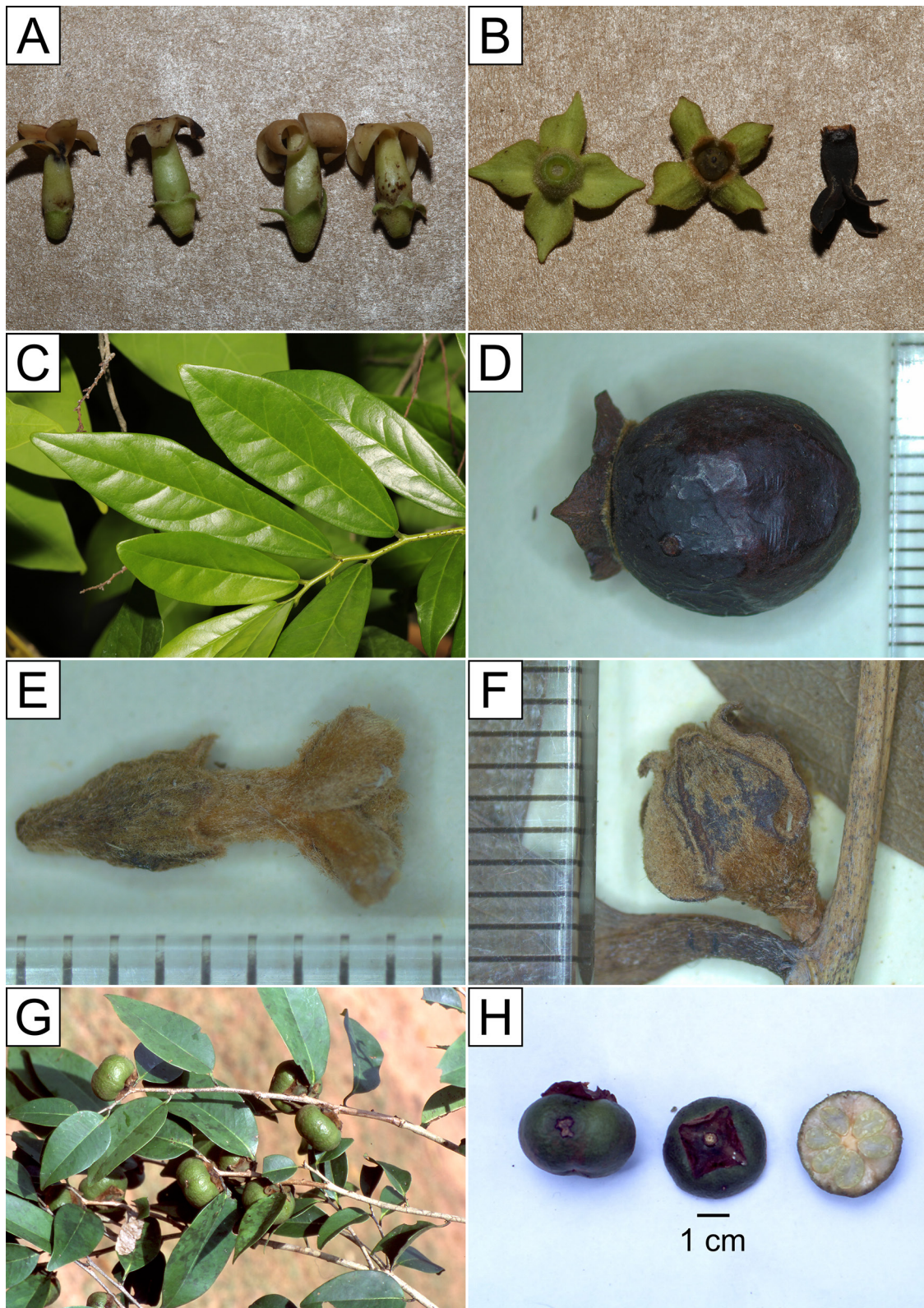
Fig. 4. A–D. Diospyros bejaudii Lecomte. A. Male flowers. B. Female calyx and corolla. C. Twig with leaves. D. Fruit ( Put 3161 K[K001361559]). E–H. D. retrofracta Bakh. E. Male flower ( Kerr 10718 K[K001361567]). F. Remaining calyx of female flower ( Kerr 12697A K[K001361574]). G. Twigs with leaves and fruits. H. Fruits. Photographed by N. Meeprom and S. Duangjai.
