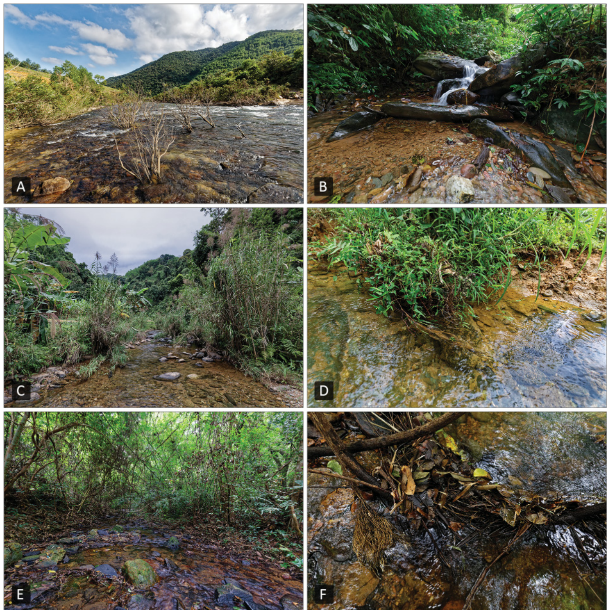
Fig. 107. Habitats of selected species of Elmomorphus Sharp, 1888. A. Vietnam, Phong Mỹ, Sông Ô Lâu River (16°31'15.3" N, 107°15'00.3" E); E. striatellus Delève, 1968 and E. siamensis Kodada, Selnekovič & Jäch sp. nov. were found in clumps of leaves and on rootlets of Neptunia sp. B. Vietnam, Thành Sơn (20°30'01.4" N, 105°06'19.3" E); E. dentipes sp. nov., and E. similis sp. nov. were found in clumps of leaves. C. Vietnam, Thành Sơn, Kho Mườìng (20°28'51.3" N, 105°07'51.6" E); E. paramontanus Kodada, Selnekovič & Jäch sp. nov., E. similis sp. nov., and E. cf. sulcatus were found on submerged rootlets of bamboo and banana trees. D. Same locality, showing submerged rootlets. E. Vietnam, Trung Mỹ (21°23'35.3" N, 105°42'52.7" E); E. cf. sulcatus was found in clumps of leaves and on submerged rootlets of bamboo, Bauhinia sp., and Sterculia lanceolata Cav. F. Same locality, clump of leaves and partly submerged rootlets.
