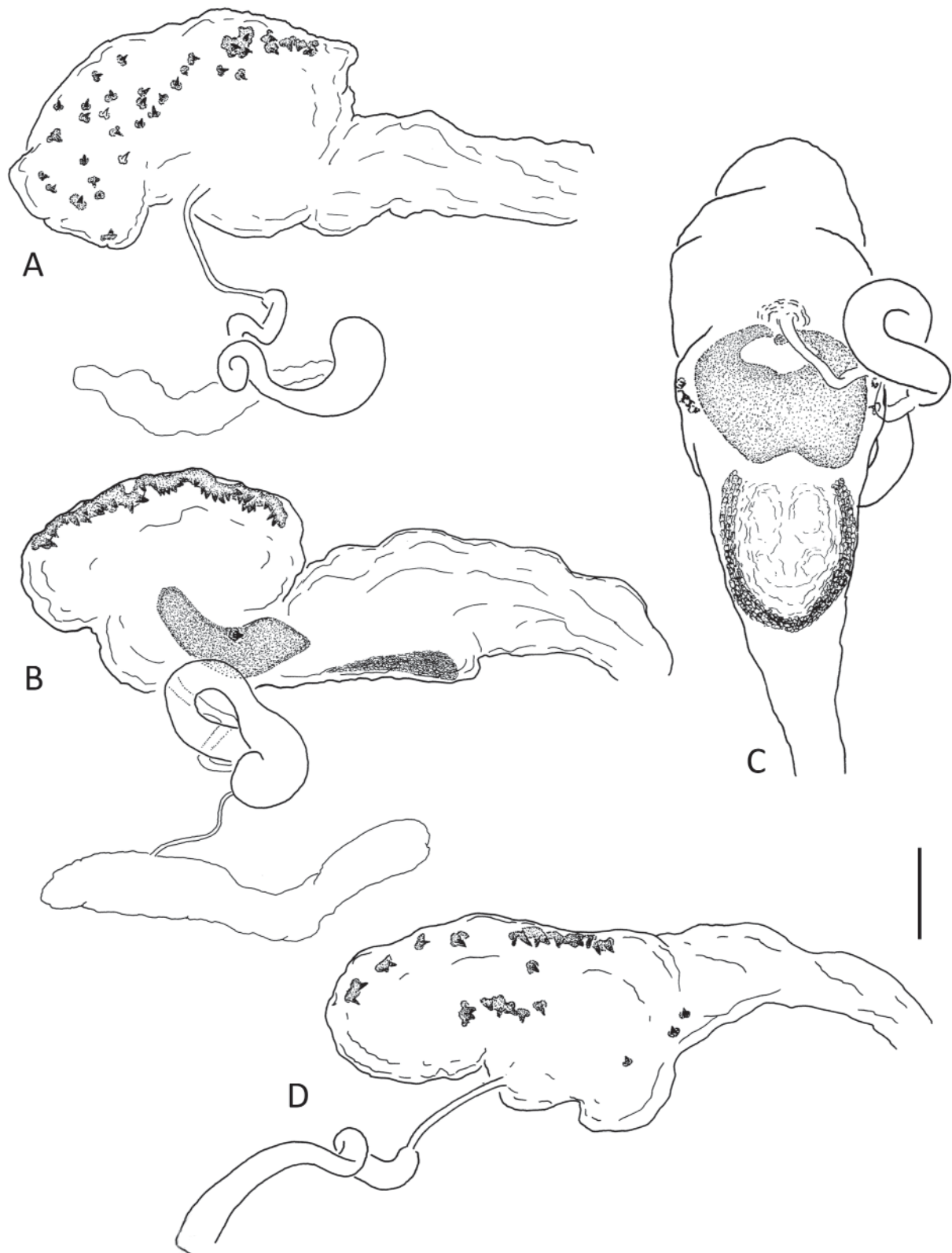
Fig. 67. Bursa copulatrix and vagina. A. Elmomorphus simplipes sp. nov., paratype from type locality (CKB). B. E. donatus Kodada, Selnekovič & Jäch sp. nov., holotype (NMW), lateral aspect. C. E. donatus , holotype (NMW), ventral aspect. D. E. paradonatus sp. nov., holotype (IAECAS). Scale bar: 0.1 mm.
