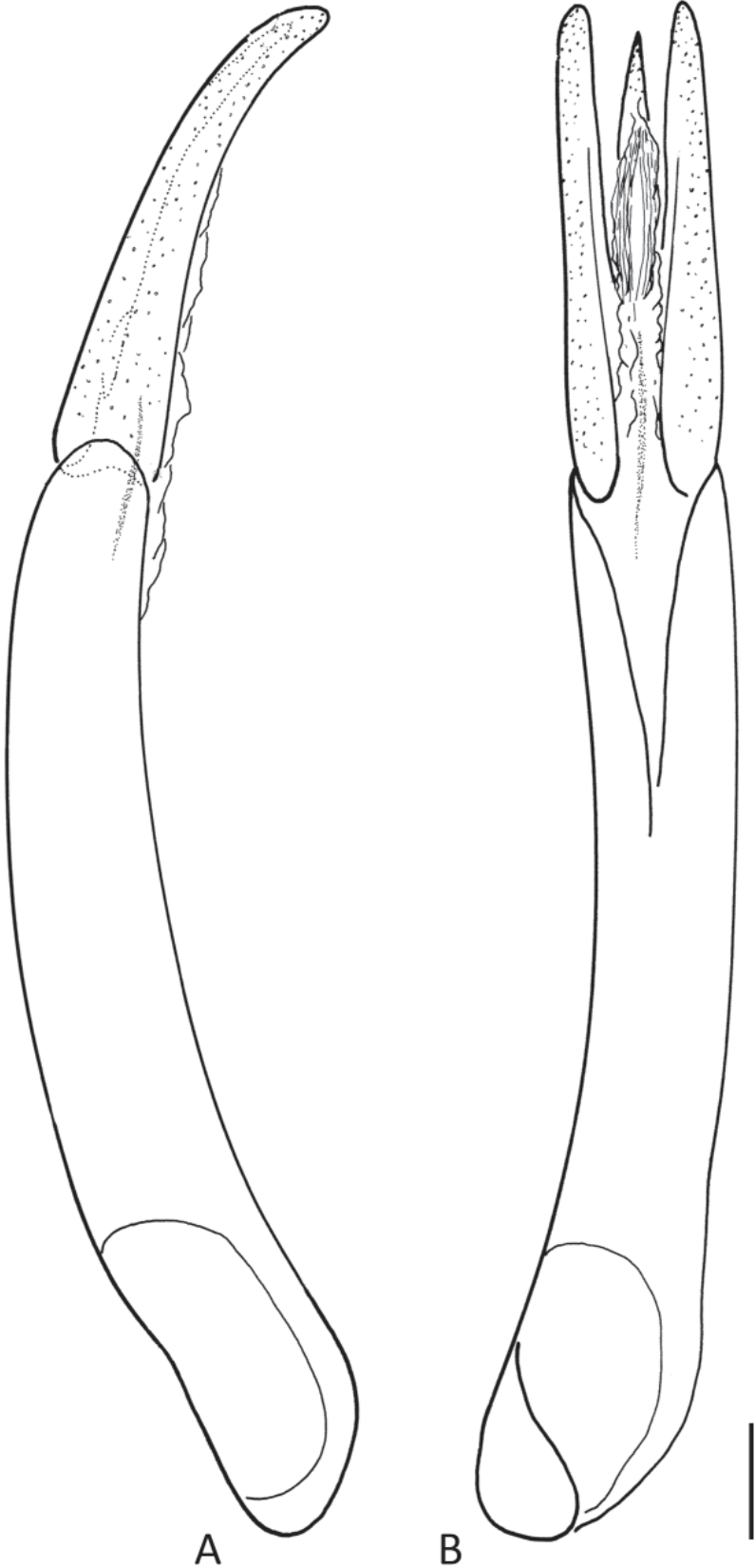
Fig. 80. Elmomorphus schillhammeri sp. nov., paratype from type locality (CKB), aedeagus. A. Lateral aspect. B. Ventral aspect. Scale bar: 0.1 mm.
