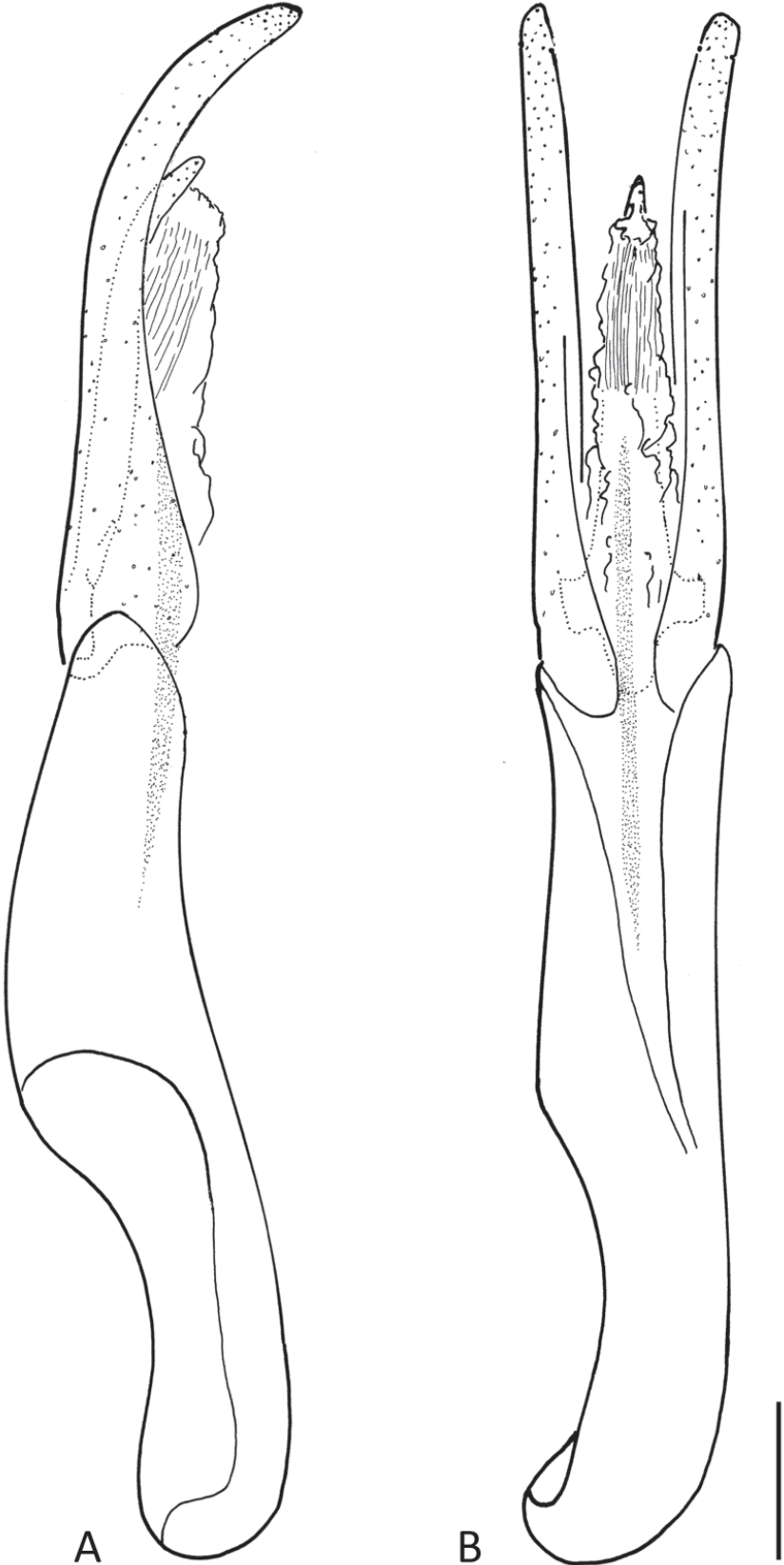
Fig. 101. Elmomorphus glabriclunis sp. nov., paratype from China, locality CWBS 49 (CKB), aedeagus. A. Lateral aspect. B. Ventral aspect. Scale bar: 0.1 mm.
