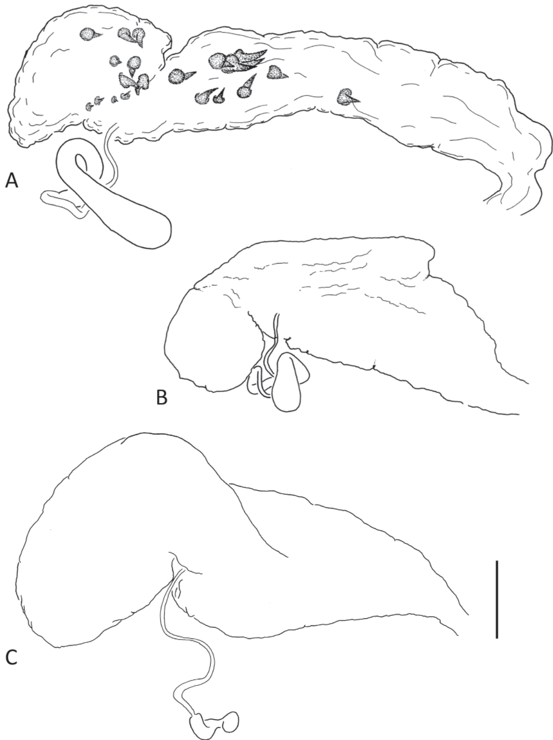
Fig. 28. Bursa copulatrix and vagina. A. Elmomorphus elmoides sp. nov., paratype from type locality (NMW). B. E. calvus sp. nov., paratype from type locality (CKB). C. E. depressus sp. nov., holotype (IAECAS). Scale bar: 0.1 mm.
