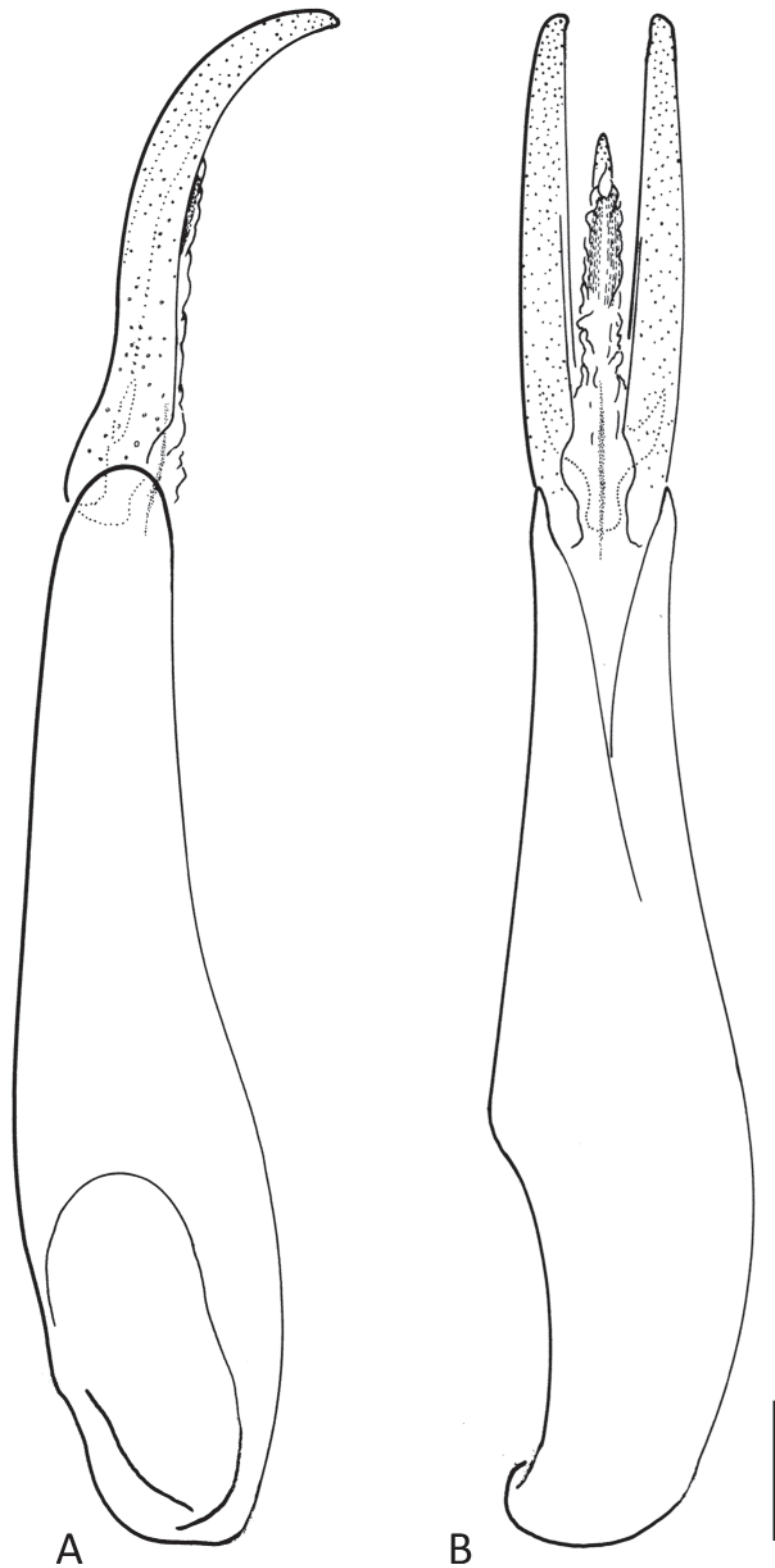
Fig. 22. Elmomorphus elmoides sp. nov., paratype from type locality (CKB), aedeagus. A. Lateral aspect. B. Ventral aspect. Scale bar: 0.1 mm.
