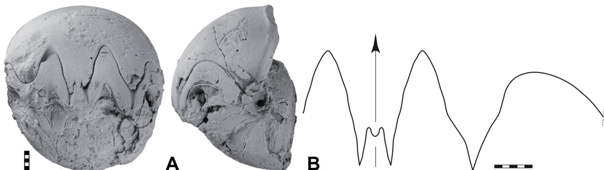
Fig. 2. Goniatices rodioni Korn & Ebbighausen, 2006, specimen MB.C.32197.1 (Korn et al. 2007 Coll.) from the Gara el Imita GI-J section. A. Ventral and lateral views. B. Suture line, at ww = 42.5 mm, wh = 23.2 mm. Scale bar units = 1 mm.
