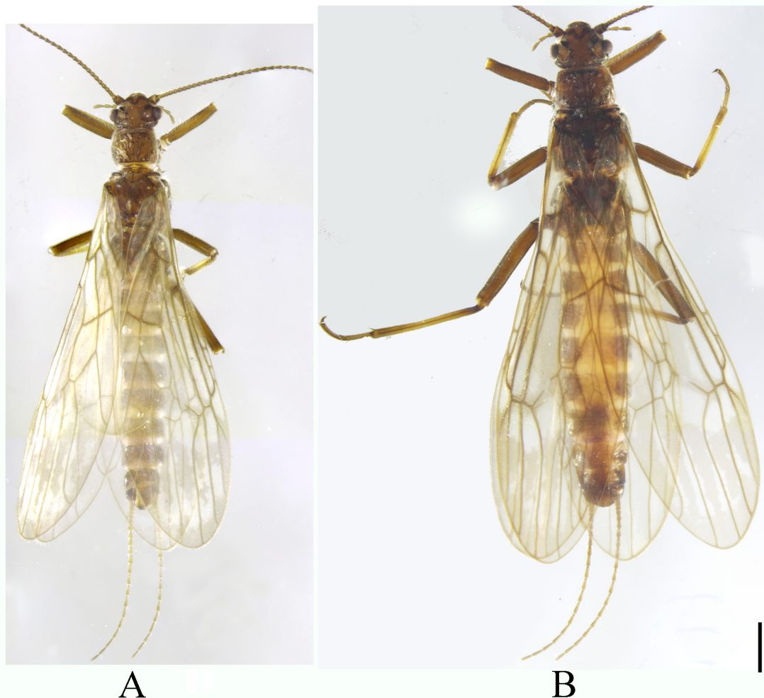
Fig. 2. Capnia s. lat. bispina Cao & Li sp. nov. A. Holotype, ♂ (HIST), habitus, dorsal view. B. Paratype, ♀ (HIST), habitus, dorsal view. Scale bar = 1 mm.
