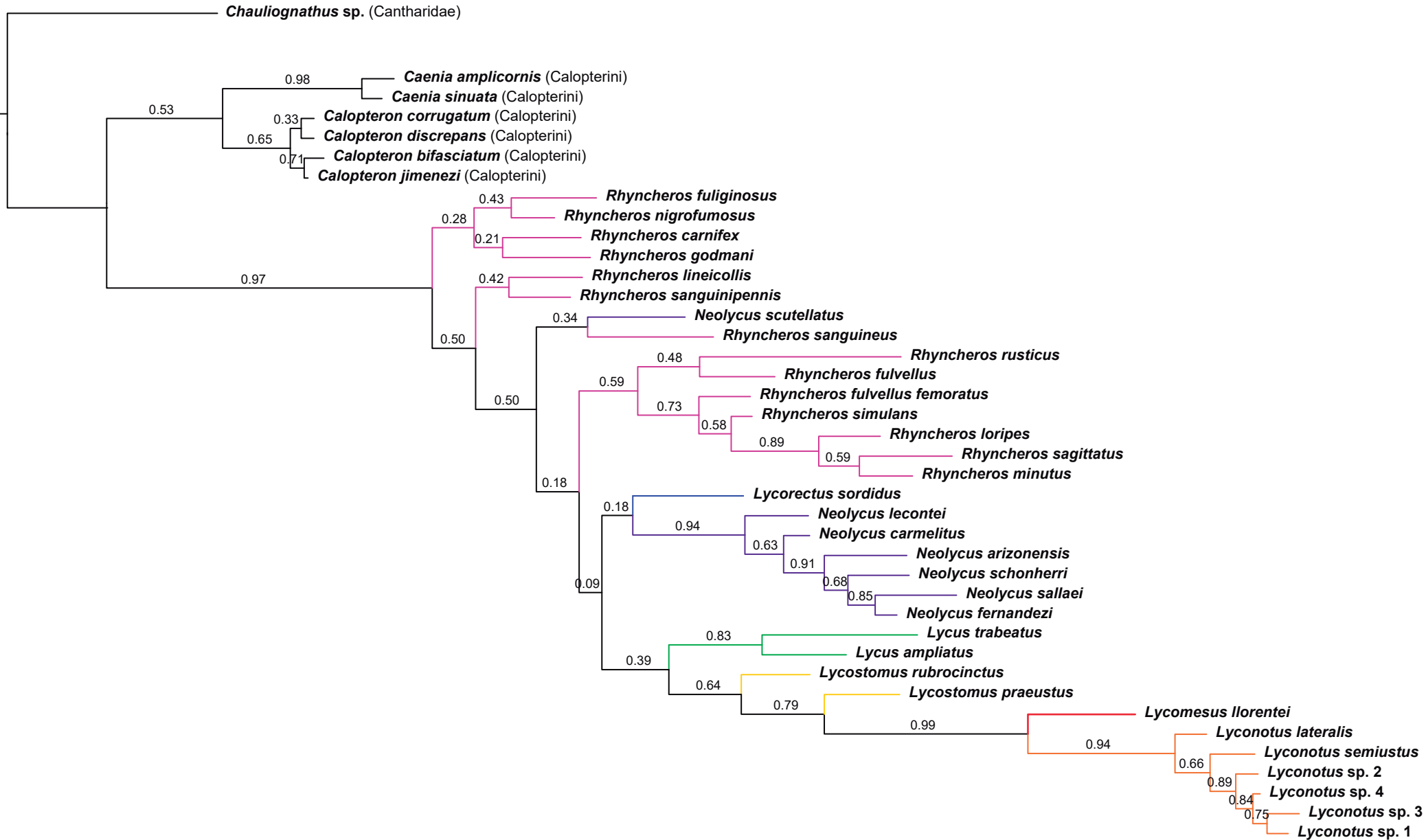
Fig. S1. Phylogenetic tree of North American Lycini, based on the Bayesian inference, node labels represent posterior probabilities (PP).
