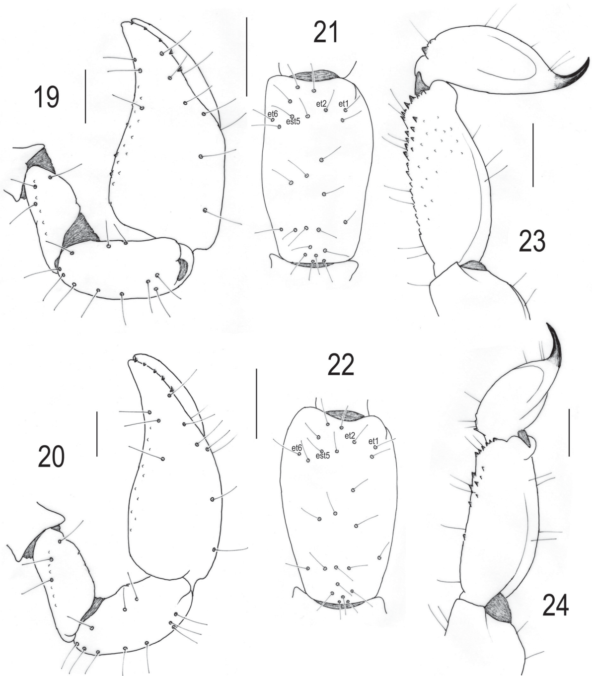
Figs 19–24. Auyantepuia manmandinan sp. nov. male holotype and female paratype from Toussaint River (MNHN). 19–22. Trichobothrial pattern. 19–20. Pedipalp, dorso–external aspects, male holotype (19) and female paratype (20). 21–22. Pedipalp patella, external aspect, male holotype (21) and female paratype (22). 23–24. Metasomal segment V and telson, lateral aspect, male holotype (23) and female paratype (24). Scale bars = 1 mm.
