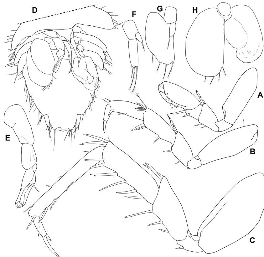
Fig. 10. Kaaetecarcinia karaja gen. et sp. nov. A–E. Paratype, ♂ (ISLA96902). A. Pereopod I. B. Pereopod II. C. Pereopod VII. D. Pleon with pleonites, pleotelson and uropods, ventral view. E. Pleopod I. F–H. Paratype, ♀ (ISLA96903). F. Pleopod I. G. Pleopod II. H. Pleopod V.
