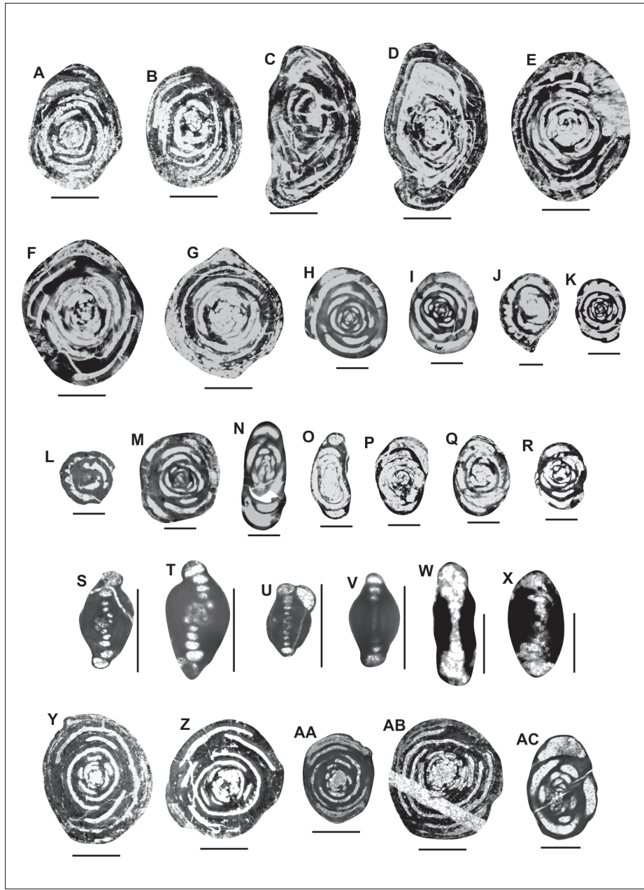
Fig. 6. Microphotographs of associated foraminiferal fauna identified in the studied Middle Permian (late Capitanian) blocks. A–B. Kamurana bronnimanni Altiner & Zaninetti, 1977. A. KDY1.6–44. B. KDY1.6–45. C–D. Globidiscus flexus Okuyucu, 2021. C. KDY1.1–5. D. KDY1.6–40. E–G. Globidiscus fragilis Okuyucu, 2021. E. KDY1.4–1. F. KDY1.4–9. G. KDY1.6–8. H–L. Baisalina akasakensis Kobayashi, 2012. H. KDY2.1–2. I. KDY2.3–13. J. KDY1.7–24. K. KDY2.2–18. L. KDY2.4–5. M. Baisalina sp., KDY2.3–10. N–O. Agathammina sp. N. KDY2.1–12. O. KDY1.5–51. P–R. Neodiscus sp. P. KDY1.8–30. Q. KDY1.7–10. R. KDY1.1–2. S–T. Midiella broennimanni (Altiner, 1978). S. KDY2.4–2. T. KDY2.4–7. U. Midiella irregulariformis (Zaninetti, Altiner & Çatal, 1981), KDY2.2–14. V. Rectogordius sp., KDY2.3–12. W. Multidiscella langei Vachard & Krainer, 2022, KDY1.3–21. X. Multidiscella zaninettiae Vachard & Krainer, 2022, KDY1.8–22. Y–Z. Hemigordiopsis luquensis (Wang & Sun, 1973). Y. KDY1.1–20. Z. KDY1.5–4. AA–AB. Hemigordiopsis renzi Reichel, 1945. AA. KDY1.6–22. AB. KDY1.6–34. AC. Glomomidiella sp., KDY2.1–33. Scale bars: A–G, Y–AB = 1 mm; H–R = 0.5 mm; S–X, AC = 0.25 mm.
