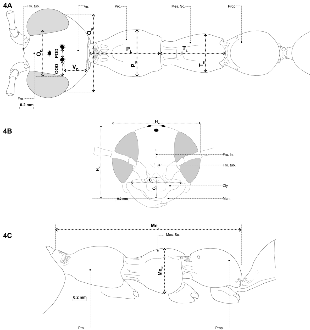
Fig. 4. Methocha hongkongensis Barthélémy & Terayama sp. nov., ♀; measurements and morphological terms. A. Dorsal habitus. B. Head frontal view. C. Lateral habitus. Abbreviations: Cly. = Clypeus; Fro. = Frons; Fro. In. = Frontal line; Fro. tub. = Frontal tubercle; Man. = Mandible; Mes. Scu. = Mesoscutellum; Pro. = Pronotum; Prop. = Propodeum; Ve. = Vertex.
