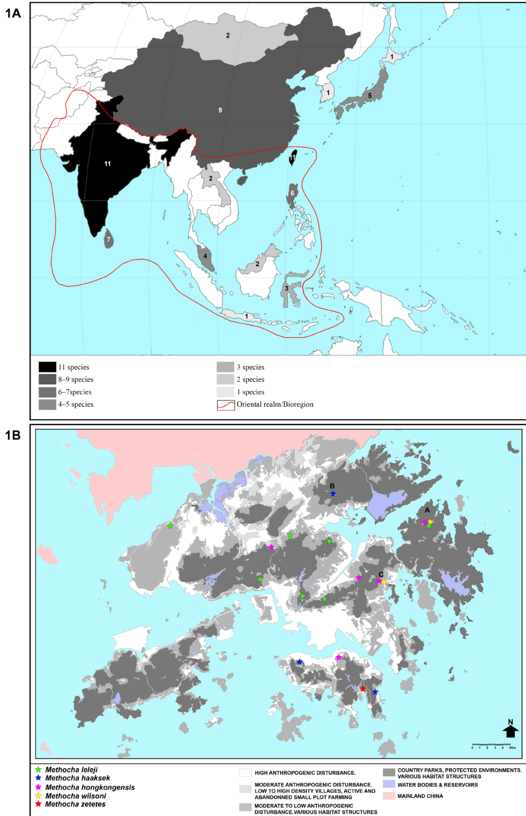
Fig. 1. Methocha spp. distribution. A. Asian distribution of Methocha spp. B. Hong Kong distribution of five species of Methocha spp.
