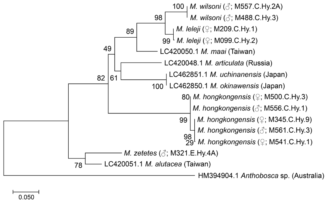
Fig. 2. Phylogenetic relationships of DNA-barcoded individuals of four species from this study. The bootstrap values are shown next to the branches. Individual specimen codes are denoted in brackets. Scale bar shows branch length in substitutions per site.
