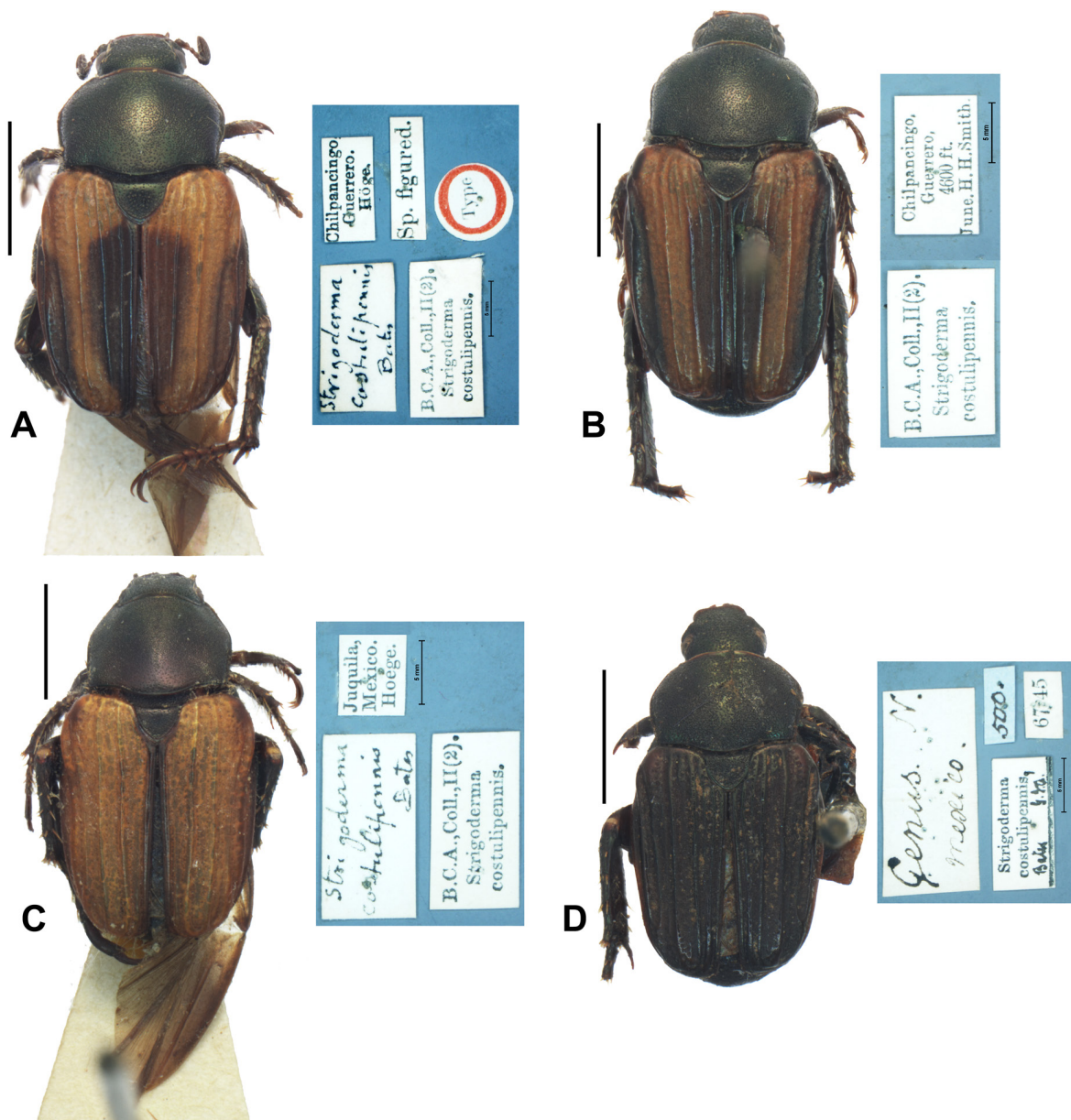
Fig. 5. Type series of Strigoderma costulipennis Bates, 1888. A. Lectotype, ♀ (here designated) (BMNH). B. Paralectotype, ♀ (here designated) (BMNH). C. Strigoderma (Costatergus) sp., ♀ (BMNH). D. Strigoderma (Costatergus) grossipennis Andalco-Cid & Ramírez-Ponce subgen. et sp. nov., paratype, ♂ (BMNH). Scale bars = 2 mm.
