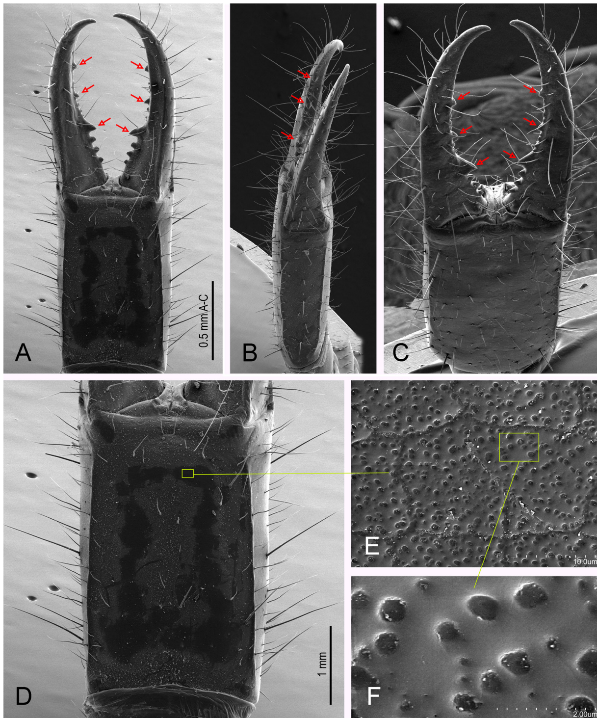
Fig. 10. Laolaojapyx chloae Sendra & Lips gen. et sp. nov., holotype, ♀ (MUVHN ZE10010). Cerci and urite X observed under electron scanning microscope. A. Cerci and urite X, dorsal view. B. Cerci and urite X, lateral view. C. Cerci and urite X, ventral view. D. Urite X, dorsal view E–F. Details of the dorsal cuticle of urite X. Red arrows indicate the positions of the three pairs of teeth.
