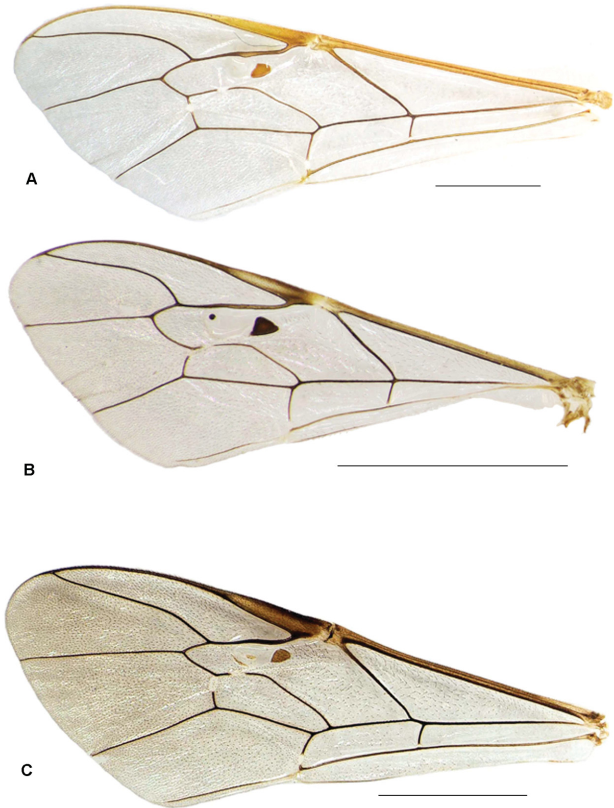
Fig. 24. Fore wing. A. Enicospilus grandiflavus Townes & Townes, 1973. B. E. mirabilis Soliman & Gadallah sp. nov. C. E. nervellator Aubert, 1966. Scale bars = 2.5 mm.
