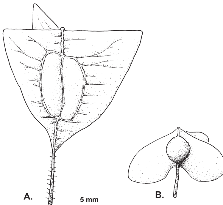
Fig. 64. Mature fruit from the types of A. B. wengeri C.E.C.Fisch. B. B. surculigera . Drawn by Rebecca Camfield. A from Wenger 324 (K); B from Kurz s.n. (K000761405).
