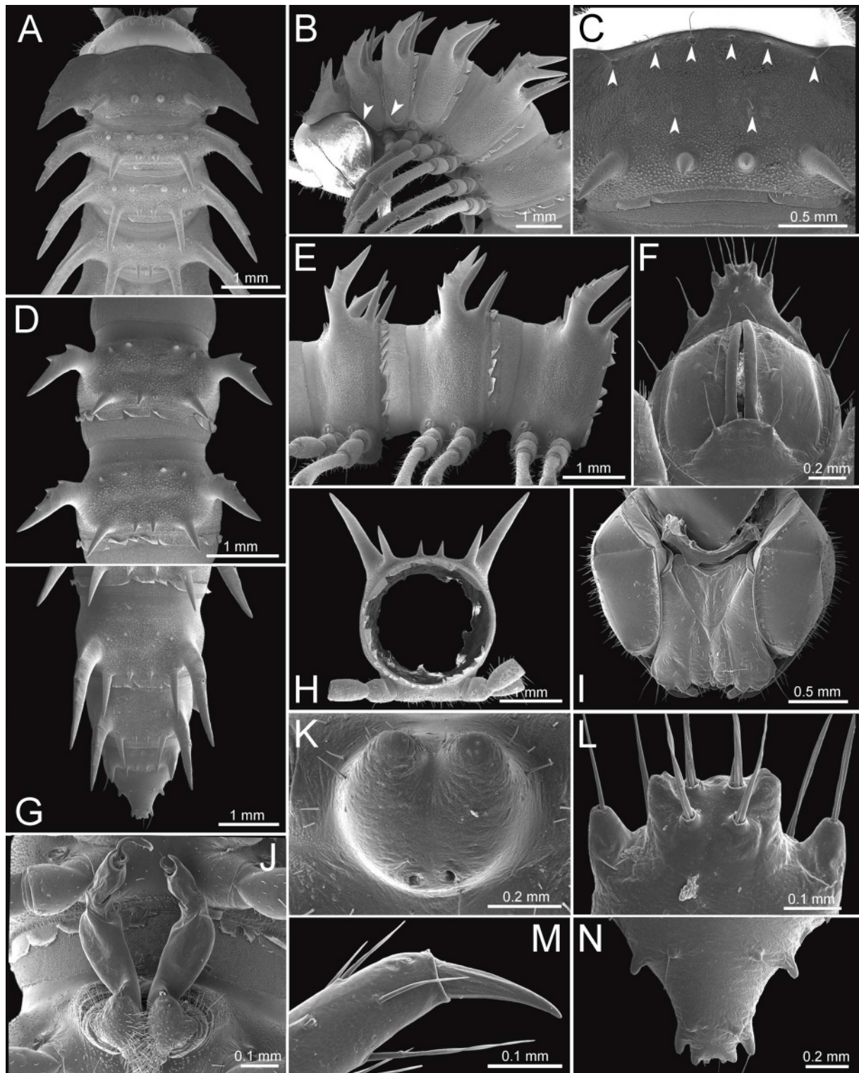
Fig. 3. General body characters of Nagaxytes Srisonchai , Enghoff & Panha gen. nov. ( N. erecta Srisonchai, Enghoff & Panha gen. et sp. nov., specimen from Prang Ka Sri Temple, Thailand), SEM images. A–B. Anterior body part (arrowheads point to pleurosternal carinae). C. Collum (arrowheads point to the setae/tubercles of the anterior and intermediate rows). D. Body rings 9–10. E. Body rings 8–10. F. Telson. G. Posteriormost rings and telson. H. Body ring 10. I. Mouth parts, ventral view. J. Gonopods in situ . K. Sternal lobe between male coxae 4. L, N. Tip of epiproct. M. Tarsus and claw of leg 13.
