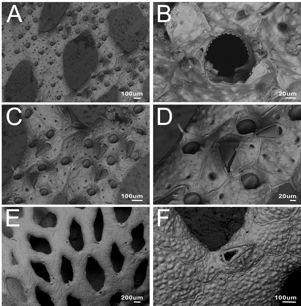
Fig. 11. Schizoretopena sp. nov. (= S. imperati sensu O’Donoghue & de Wateville 1939), from Schizoretopena imperati , coll. O’Donoghue (NHMUK 1963.9.4.12). A. Colony view. B. Primary orifice showing distal denticles and proximal condyles. C. Autozooids with giant avicularia. D. Large vicarious avicularia on cystid. E. Abfrontal view. F. Detail of abfrontal avicularium and rugose surface.
