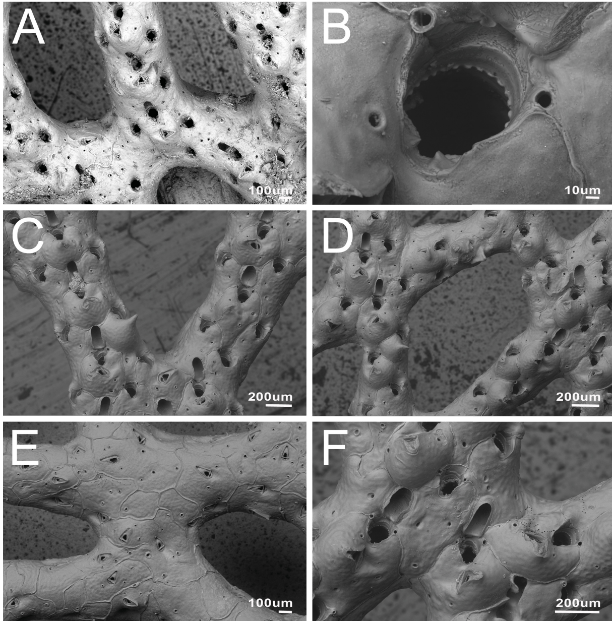
Fig. 8. Schizoretepora imperati (Busk, 1884). A from Retepora imperati , syntype (NHMUK 1963.2.12.202); B–F from Retepora imperati , syntype (NHMUK 1934.2.16.23). A. Colony, frontal view. B. Primary orifice, detail. C–D. Ovicellated autozooids with giant avicularia. E. Detail of ovicellated autozooid with giant avicularia. F. Abfrontal view with triangular avicularians.
