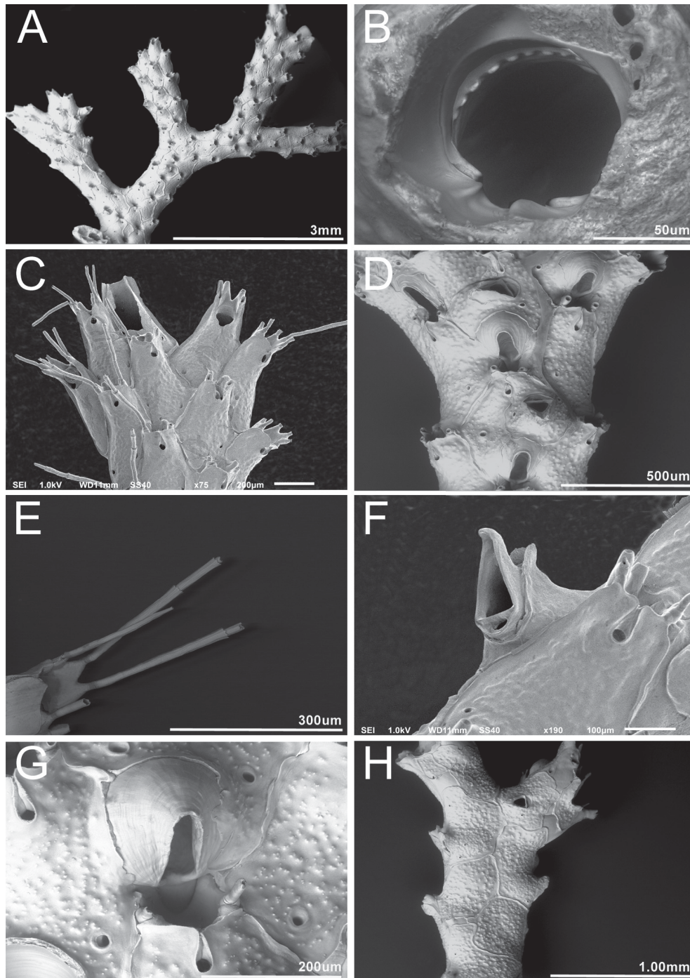
Fig. 5. Schizoretepora solanderia (Risso, 1826), Menorca Channel (A–B, D, G–H: MZB 2014-1471; C, E–F: MZB 2014-1486). A. Colony view. B. Detail of aperture. C. Growing margin with autozooids showing up to six spines. D. Older ovicellate autozooids with giant vicarious avicularia. E. Detail of articulated and crenated spines. F. Marginal avicularia showing nested piling of cystids. G. Details of ovicell. H. Abfrontal view with avicularia.
