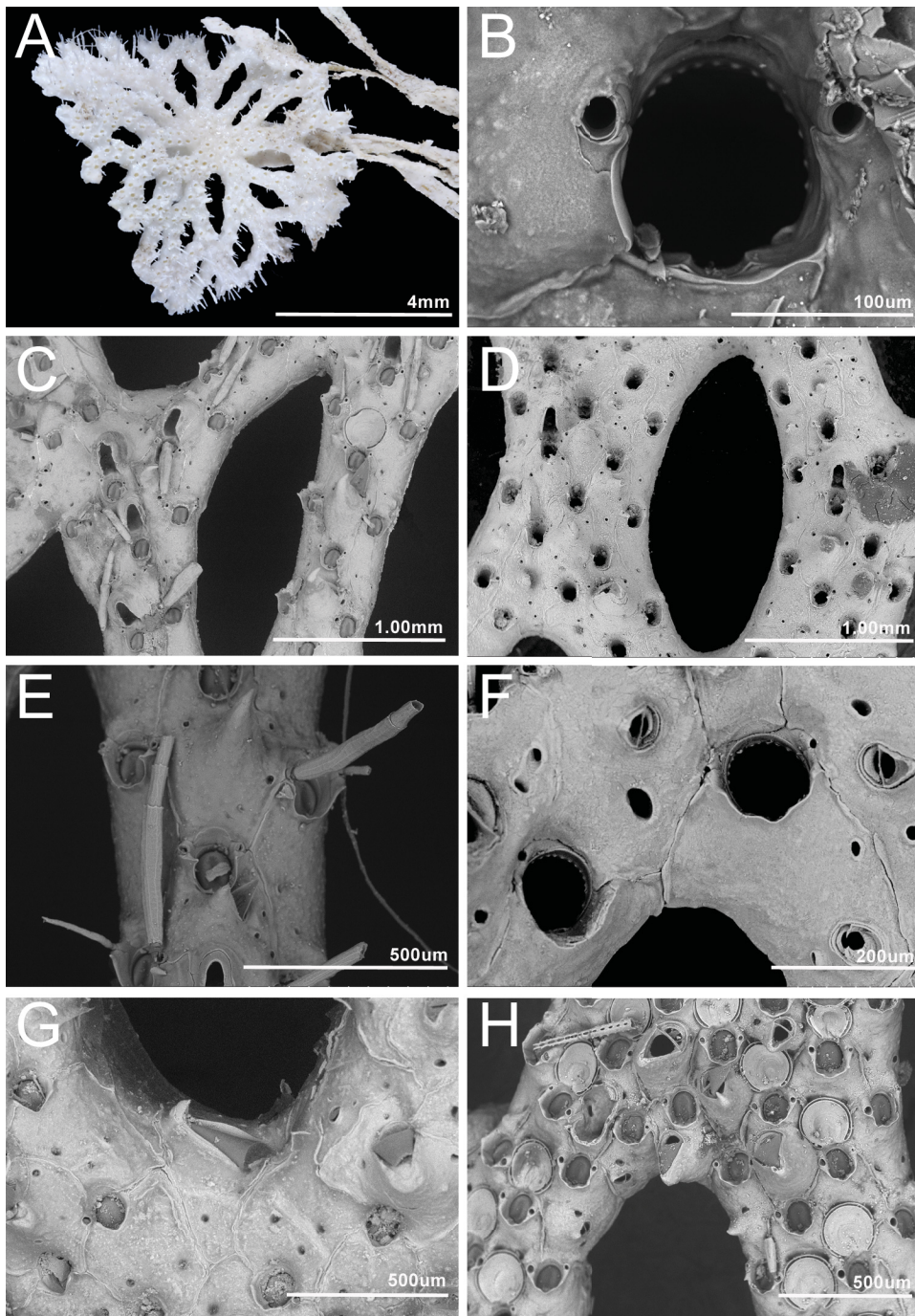
Fig. 9. Schizoretepora pungens (Canu & Bassler, 1925). A from specimen labelled as Schizellozoon longisetae , Gautier leg. (MNHN-IB-2008-11127); B, H from specimen labelled as Retepora imperati , coll. Canu (MNHN-IB-2014-29); C from specimen labelled as Schizellozoon longisetae (MNHN-IB-2008-14462); D from Schizoretepora pungens , holotype, coll. Canu (MNHN-IB-2014-20); E from Schizoretepora pungens (MNHN-IB-2008-14434); F from specimen labelled as Retepora imperati (MNHN-IB-2008-982); G from specimen labelled as Retepora imperati , coll. Calvet (MNHN-IB-2008-6052). A. Young colony with spines. B. Primary orifice showing distal denticles, proximal condyles, sinus and smothered peristome. C. Young autozooids showing spines and acute peristomes. D. Old autozooids lacking spines and with smothered peristomes. E. Detailed view of articulated and carenated club-like spines. F. Adventitious triangular (upper side) and oval (bottom right) avicularians. G. Giant avicularium at basis of fenestra. H. Giant avicularia on large cystids showing crossbar without columella.
