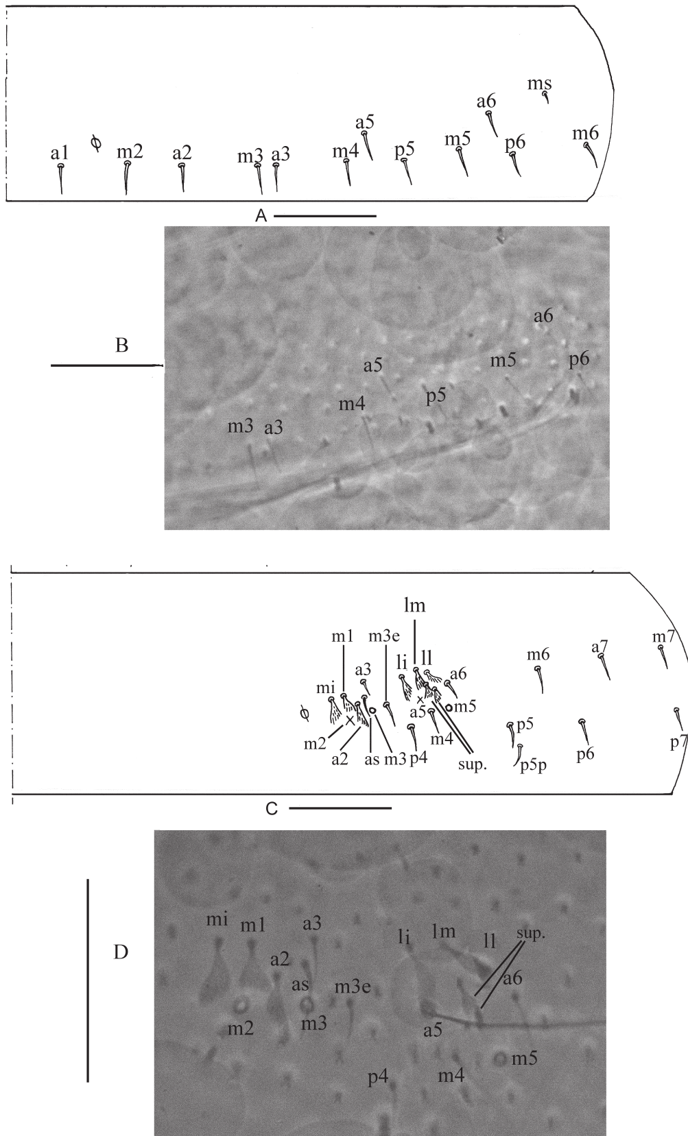
Fig. 5. Lepidocyrtus (A.) huizhouensis sp. nov., dorsal chaetotaxy (right side). A–B. Abd. I. C–D. Abd. II. Scale bars: 50 μm.
